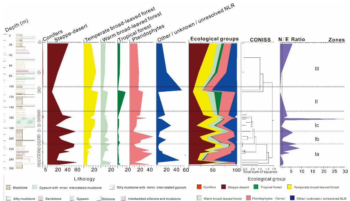
Figure 3: Cumulative pollen summary diagram of the Ria Zhong (RZ) section in the Nangqian Basin, Yushu area, Tibet, with palynomorph percentages of the total pollen sum plotted on the x-axis, and zones and subzones based on CONISS ordinations. Pollen taxa are grouped in Plant Functional Types (PFTs) according to their correspondence with nearest living relatives (NLR), indicated in the legend. Some taxa have multiple or unresolved botanical affinities, and are thus assigned to the “Other / unknown / unresolved NLR” group. Productive horizons are indicated by a small trilete spore to the right of the simplified section log. The Nitraria/Ephedra (N/E) pollen ratio is plotted in purple, with a dashed line indicating the transition point between desert/semi-desert ecosystems (< 1) and steppe-desert (> 1).
