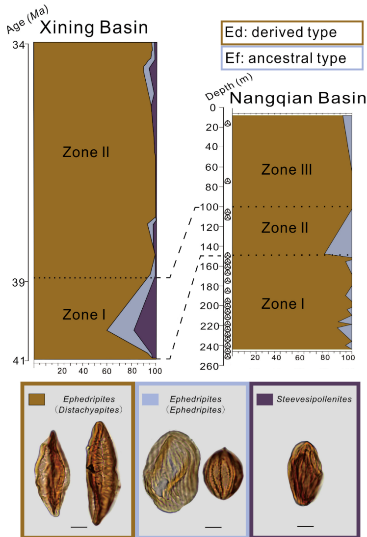
395 Figure 5: Eocene ephedroid pollen composition in the Xining (northeastern TP) and Nangqian (east-central TP) 396 basins, illustrating the distributions of Ephedripites subgen. Ephedripites (ancestral type; “Ef”), Ephedripites subgen. 397 Distachyapites (derived type; “Ed”), and Steevesipollenites . Productive horizons for the Ria Zhong (RZ) section are 398 indicated by a small trilete spore to the right of the marked depths.
