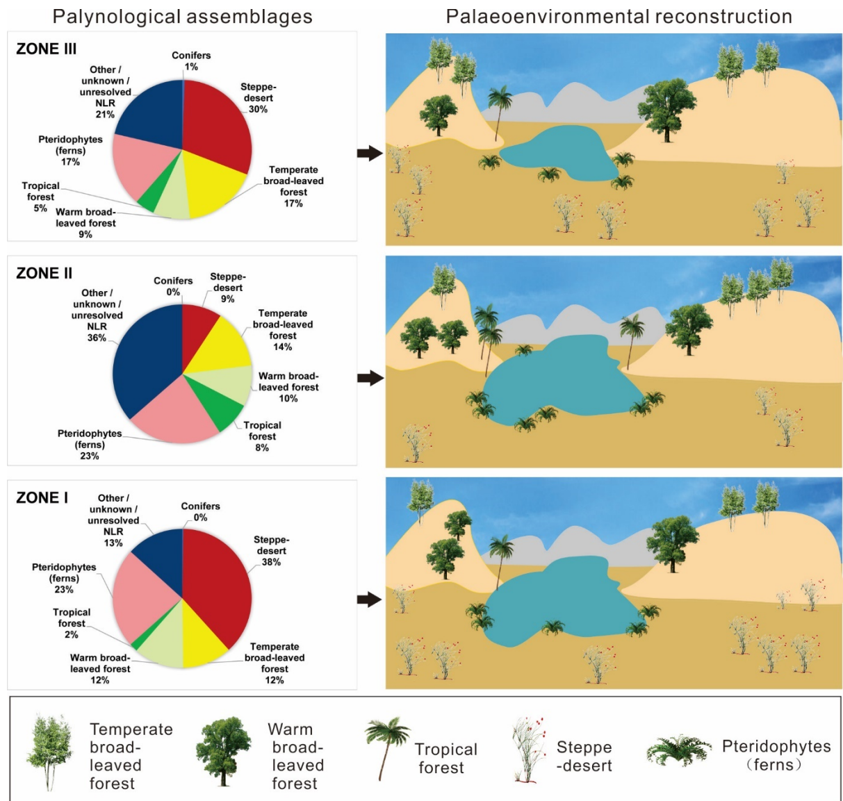
Figure 6: Palaeoenvironmental reconstruction of the Nangqian area, illustrating the three distinct floral assemblages recovered from the RZ section. Vegetation during deposition of Zone I was dominated by steppe-desert shrubs, which decreased sharply in Zone II in conjunction with a spike in tropical forest. Afterwards the basin became drier and steppe-desert vegetation again dominated the landscape.
