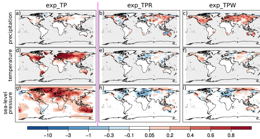
Figure 6. Summer season RMSESS values of exp_TP (a, d, g), exp_TPR (b, e, h) and exp_TPW (c, f, i). x^f is the ensemble mean of the CCC400 model simulations when the RMSESS values calculated for the exp_TP experiment, while x^f was replaced with the analysis mean of the exp_TP for the other two experiments.
