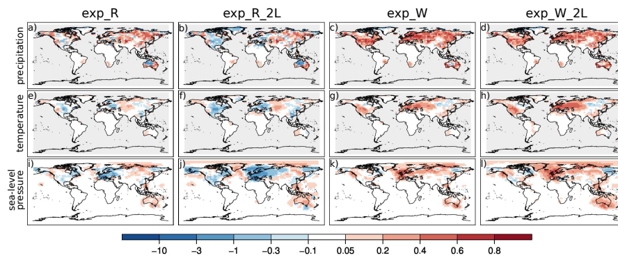
Figure 4. Summer season RMSESS values of precipitation (a, b, c, d), of temperature (e, f, g, h), and of sea-level pressure (i, j, k, l) by assimilating only precipitation amounts (a, e, i), only precipitation amounts with doubled localization length scale parameter (b, f, j), only number of wet days (c, g, k), and only number of wet days with doubled localization length scale parameter (d, h, l).
