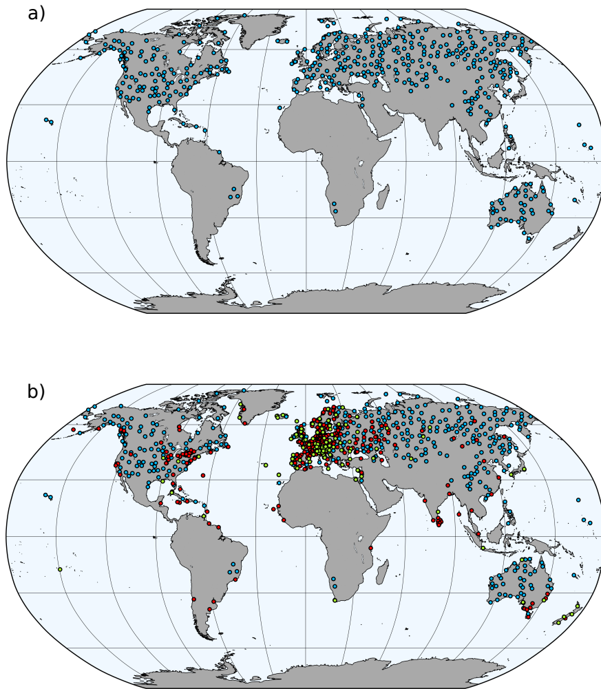
Figure 1. The location of precipitation observations (a) used in exp_R , exp_W , exp_R_2L , and exp_W_2L experiments. The location of instrumental precipitation (blue), temperature (red), sea-level pressure (green) observations (b) assimilated in exp_TPR and exp_TPW experiments.
