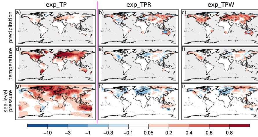
Figure 6. Summer season RMSESS values of exp_TP (a, d, g), exp_TPR (b, e, h) and exp_TPW (c, f, i). \mathbf{x}^f is the ensemble mean of the CCC400 model simulations when the RMSESS values calculated for the exp_TP experiment, while \mathbf{x}^f was replaced with the analysis mean of the exp_TP for the other two experiments.
