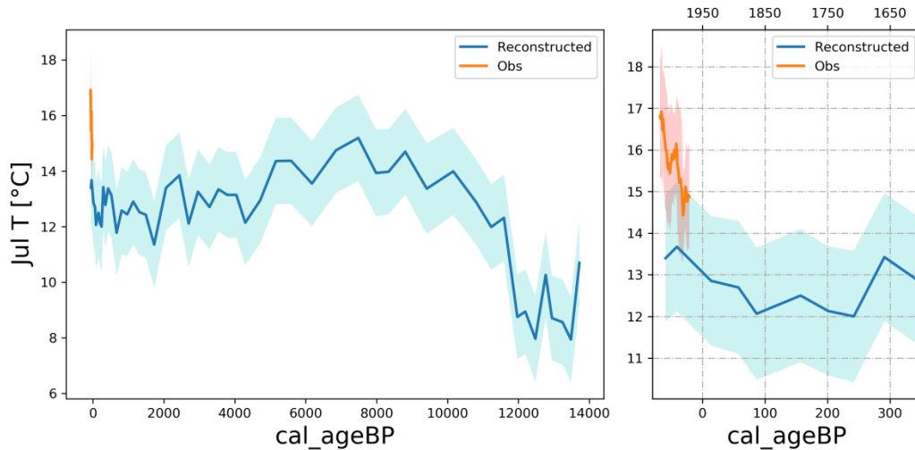
Figure 8. Comparison of current data and reconstructed July mean temperature at the Lake Verdarolo site (see Fig. 1 for location). The blue line is the reconstructed temperature and the shaded area is the sample-specific estimated standard error associated with the temperature reconstruction based on chironomid assemblage from Samartin et al. (2017). The orange line represents the July mean temperature (1961-2018) retrieved for the grid cell of Lago Verdarolo from Emilia-Romagna climate reanalysis ERACLITO (11 years running average). The shaded orange area is +/- one standard deviation. The full available period is reported on the left, while a zoom on the most recent period (since 1600 AD) is shown on the right.
