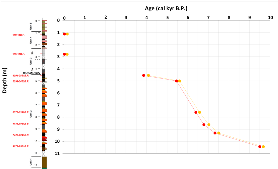
400 Figure 6. S1 core stratigraphy and the age-depth model obtained from radiocarbon dates. Red and orange lines represent the two-sigma probability envelope.
