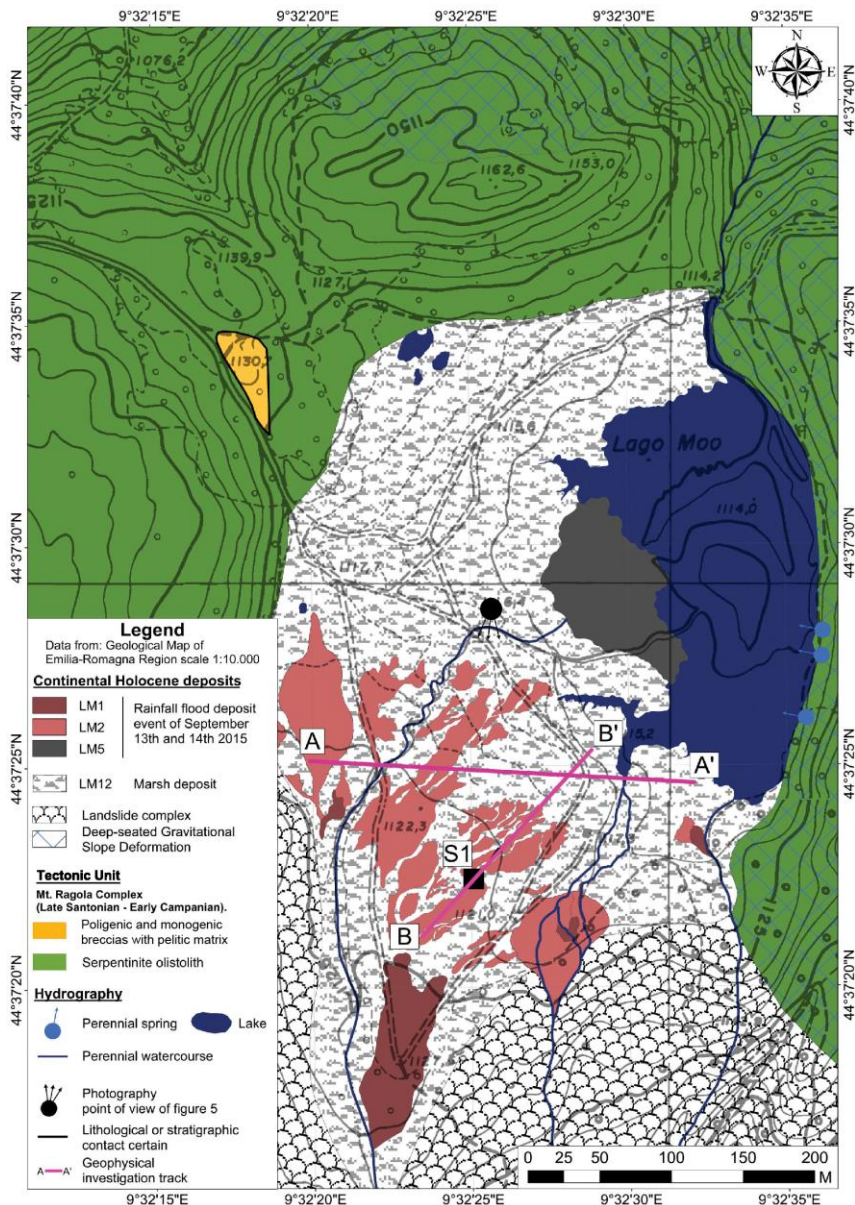
Figure 2. Geomorphological map showing the main geological units and the hydrological elements of the Lake Moo plain. The detailed mapping of flood deposits formed during the recent HIP event (13 th -14 th September 2015), the location of the geognostic investigations and the geophysical surveys tracks are also reported. Original data from field campaign overlaid on the Geological database of Emilia-Romagna region.
