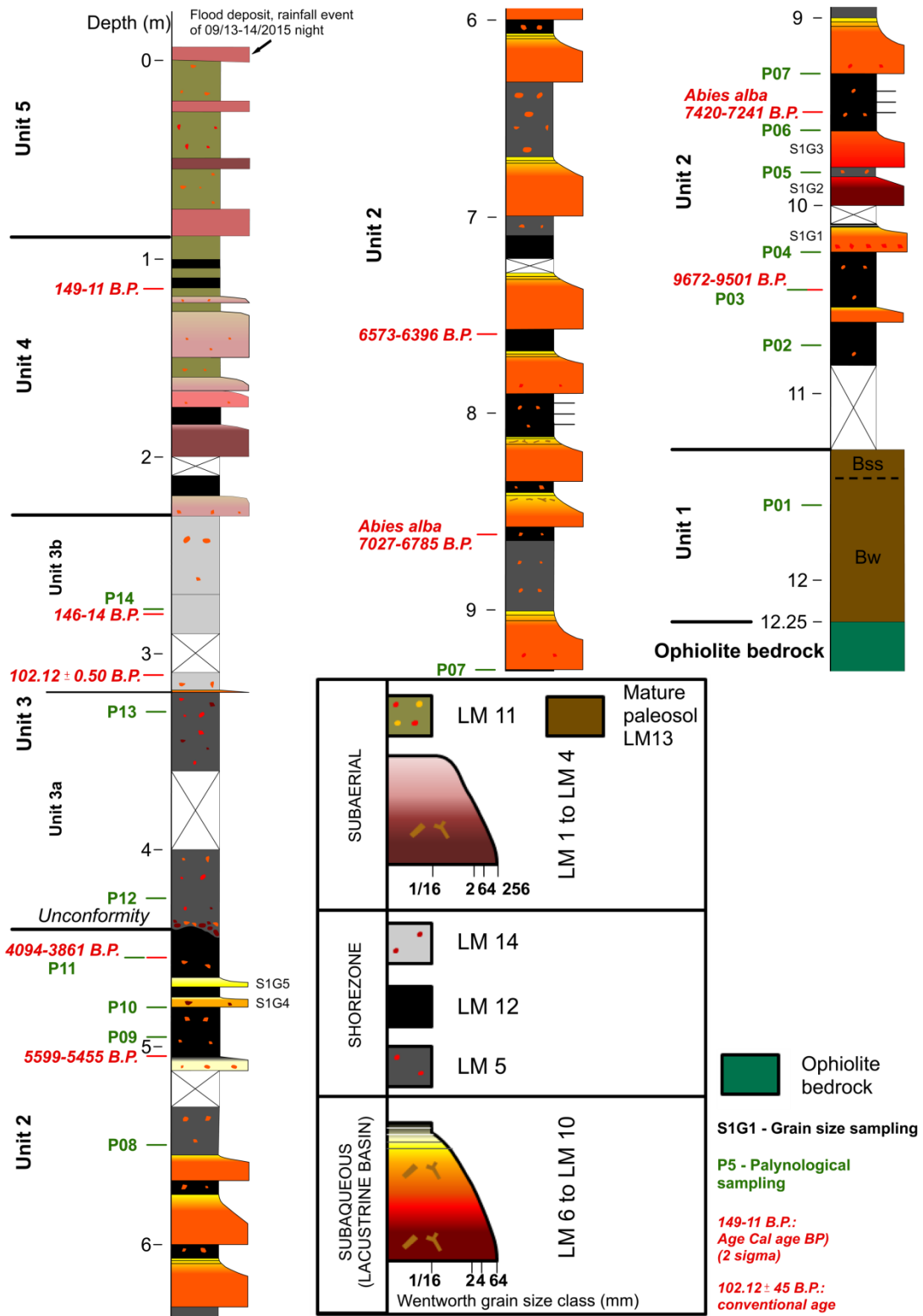
Figure 3. Sedimentological features and lithofacies characterisation of the reference core S1. Radiocarbon dates, palynological and grain-size samples as well as stratigraphic units (described in the section 4.2.) are also reported.
