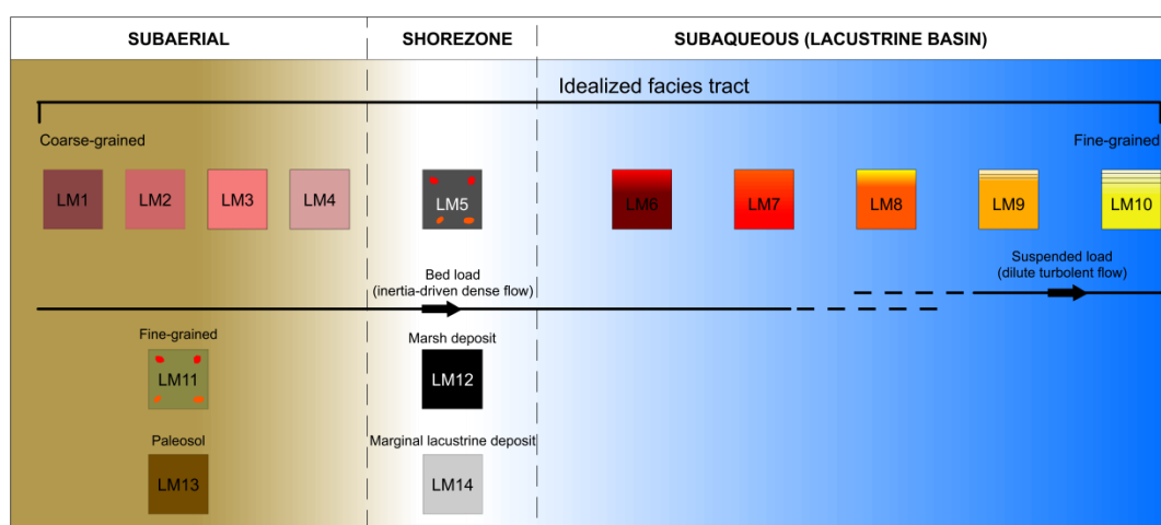
Figure 4. Idealised genetic facies tract showing the fourteen lithofacies (LM1-LM14) identified within the reference core S1, whose stratigraphy is reported in Fig. 3.
