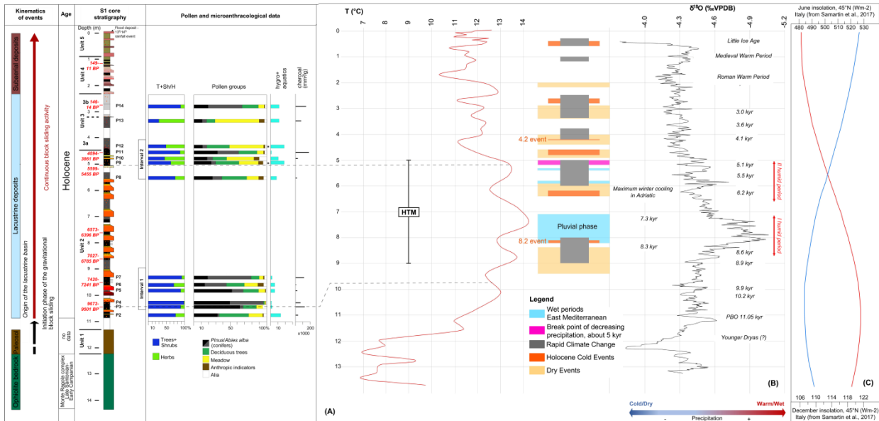
Figure 7. Stratigraphy of core S1, main palynological features and microcharcoal content. Relative abundances of pollen groups explained in the text (sub-section 3.3), are reported along with the frequencies of hygrophilous herbs and aquatics. Asterisks point to samples containing coprophilous fungi and other spores like Sporormiella , Dicrocoelium and Ascaris . These data are compared with the most relevant paleoclimate reconstructions available from literature for the area of interest. Panel (A) Reconstructed mean July air temperature from Lago Verdarolo (from Samartin et al., 2017); Panel (B) \delta^{18}\text{O} speleothem records and reconstructed precipitation trends (mean anomaly time series) from Corchia cave (slightly modified from Combourieu et al., 2013; Zanchetta et al., 2011; Zhornyak et al., 2011) and Panel (C) June (red) - December (blue) insolation values reported for 45° Nord (from Samartin et al., 2017). Main Holocene climate phases and events are also shown (Regattieri et al., 2014). Available radiocarbon ages are reported as calibrated years BP.
