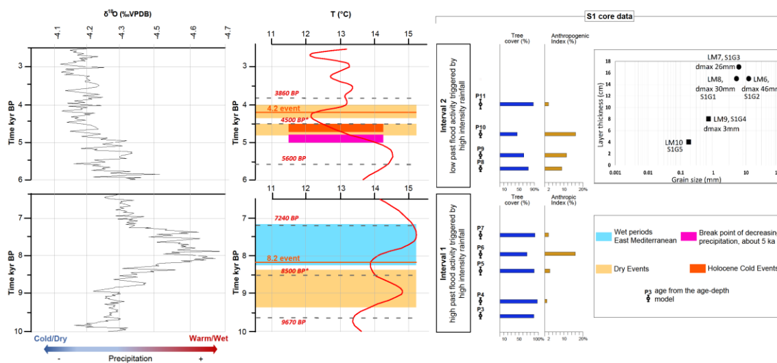
Figure 10. Sedimentological and palynological features of two key stratigraphic intervals (Intervals 1 and 2) from the reference core S1. These features are compared with the most relevant paleoclimate data available from literature for the area of interest (for references, please see Figure 7). The Anthropogenic Index (AI) has been calculated as: (Anthropogenic indicator/tree percentage) * 100 following Accorsi et al. (1999). Asterisks point to samples containing coprophilous fungi and other spores like Sporormiella , Dicrocoelium and Ascaris . Core S1 sample ages derive from the age-depth model reported in Figure 6. P samples correspond to the pollen samples; LM labels refer to the lithofacies explained in text (section 4.1.) and in Figures 3-4; dmax corresponds to the maximum diameter.
