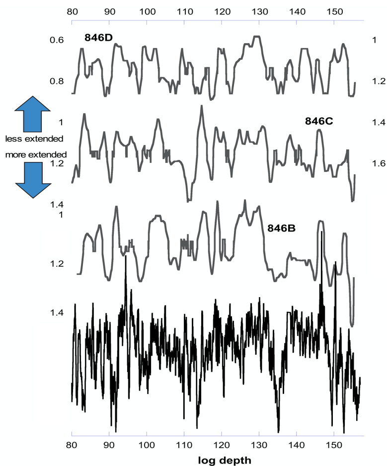
Figure 3. Coring distortion inferred from Match alignment of GRAPE composite sections to the borehole conductivity log (log has been inverted, detrended, and normalized) generated using the “smooth” Match parameters emphasizing a 1:1 depth mapping of core data to the downhole log. Values >1 indicates stretching of the cored section relative to the borehole log, which we assume represents the best representation of the in situ stratigraphy. Note that the scale for coring distortion has been inverted so that higher expansion (stretching) is in the downward direction.
