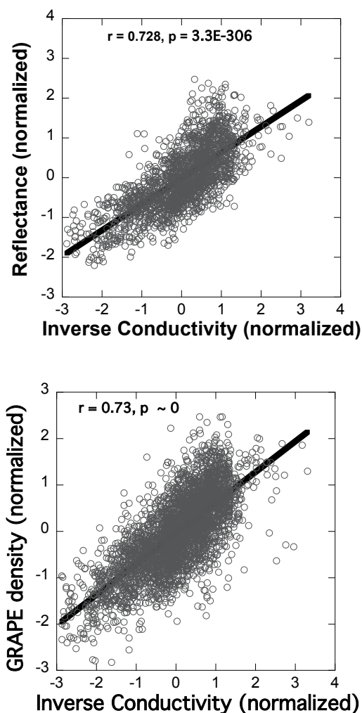
Figure 1. Correlations of the inverse of borehole log conductivity (detrended and normalized) to GRAPE density (detrended and normalized) and to color reflectance (channel 1, detrended and normalized) over the depth interval 85-170 mbsf (95-181 mcd), hole 846B. Note that the inverse of conductivity is plotted. Both correlations ( N = 1853, 3388 ) are highly significant. Correlations of the same variables from holes 846C and 846D were very similar
