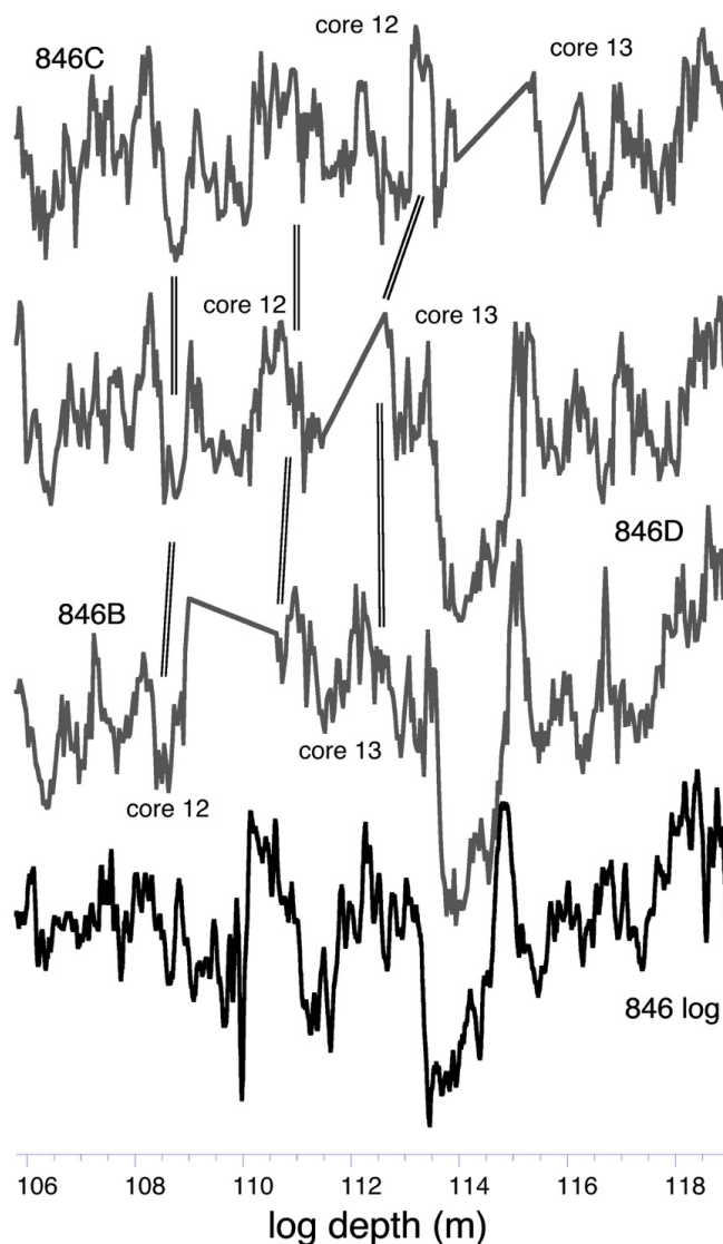
Figure 6. Detail of reflectance-based correlations (original mcd 122.6-137.8) of offset holes 846B, 846C, and 846D correlated to the common depth scale of the borehole log (log depth 106-119 m). Signals were detrended and normalized; higher reflectance and lower conductivity plot upward. Note the problematic tie of the base of Hole 846C, core 12 to the top of Hole 846D, core 13 (shipboard splice). In contrast, Hole 846B has a sequence that correlates easily to the borehole log and can be reliably spliced to the base of Hole 846D, core 12.
