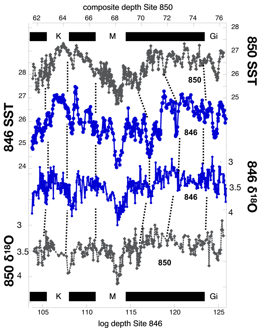
Figure 10. Comparison of the new alkenone-based SST and \delta^{18}\text{O} composites from Site 846 to composites from Site 850. The location of magnetic polarity reversals (reversed Kaena, Mammoth and Gilbert polarity zones indicated by abbreviations) at Site 850 can be mapped to Site 846 with high confidence by the close correspondence of SST patterns (note: polarity determinations are only available at Site 850).
