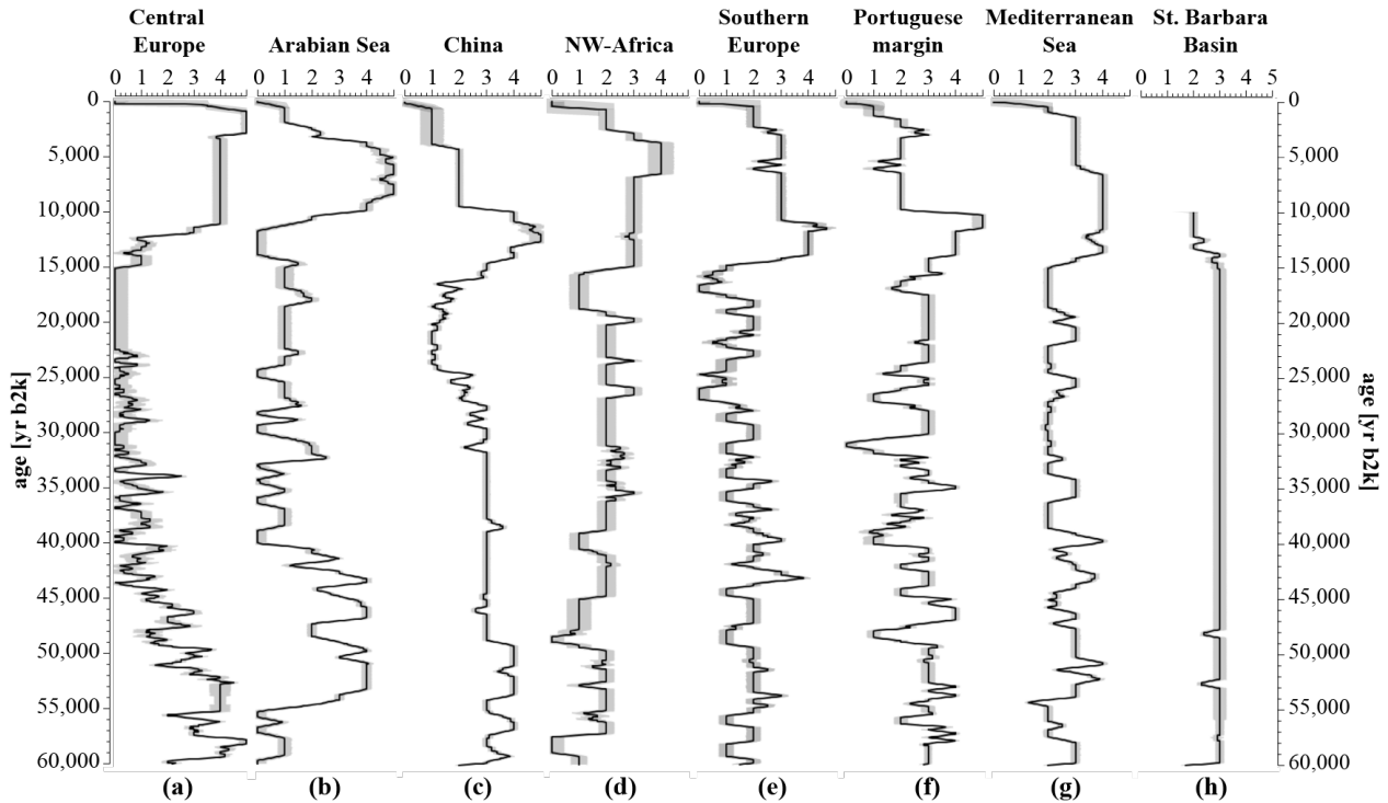
Figure 3: Aridity indices for the key regions over the last 60 000 years. Smaller values indicate more arid, higher values indicate more humid conditions. An early MIS3 wet phase and a Holocene wet phase on various timings for the regions are recognisable.
