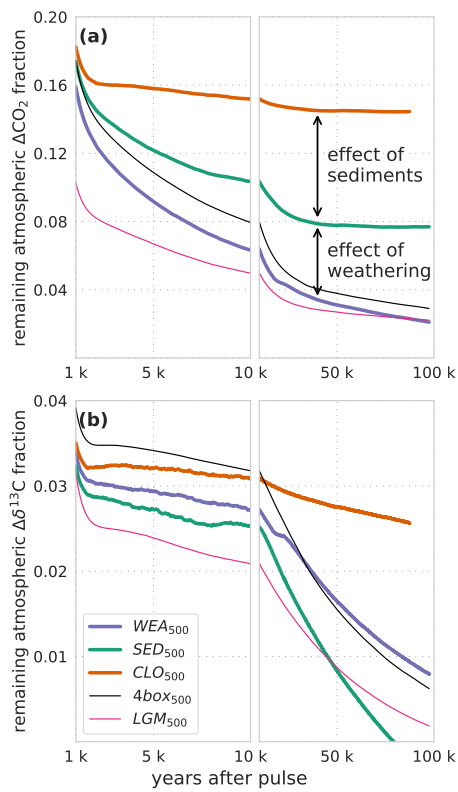
Figure 6: New Fig. 2 for the revised manuscript: (a) CO_2 and (b) \delta^{13}C perturbation in the atmosphere for the factorial simulations WEA_{500} , SED_{500} , CLO_{500} , 4box_{500} , and LGM_{500} . Shown is the time interval 1 kyr to 100 kyr. Data are filtered with a moving average of 1000 years in the interval 1 kyr - 10 kyr and 5000 years in the interval 10 kyr - 100 kyr for better visibility. Note that experiment CLO_{500} was run for 90 instead of 100 kyr.
