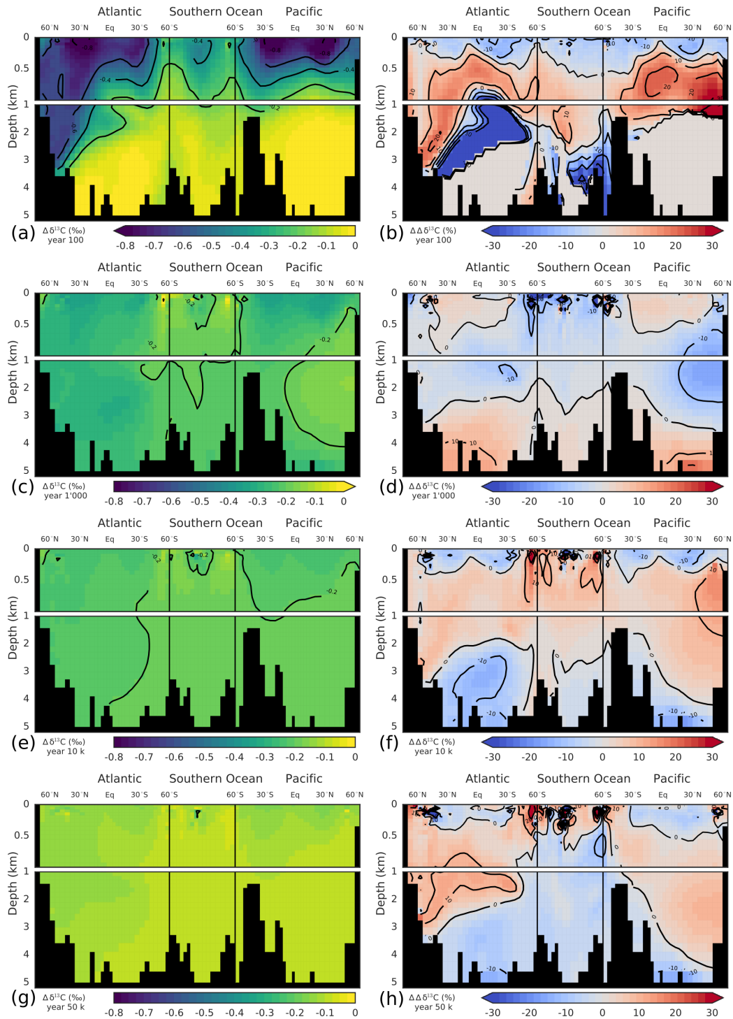
Figure 6. EOF-pattern Modeled \delta^{13}\text{C}_{\text{DIC}} perturbation in ‰ (a,c,e,g) and difference between modeled and reconstructed \delta^{13}\text{C}_{\text{DIC}} perturbation using the first three principal components. These differences are shown in ‰ of the modeled perturbation (b,d,f,h). Shown are time slices 100 years (a,b) first, 1 kyr (c,d), 10 kyr (e,f) second, and 50 kyr (g,h) third-principal-component after the pulse release of carbon. Corresponding PC timeseries are shown. Note that in panel (b) perturbation values smaller than 10.051 ‰ (abyssal Atlantic and Pacific) have been masked for better visibility as the perturbation has not yet propagated into these regions (see panel (a)).
