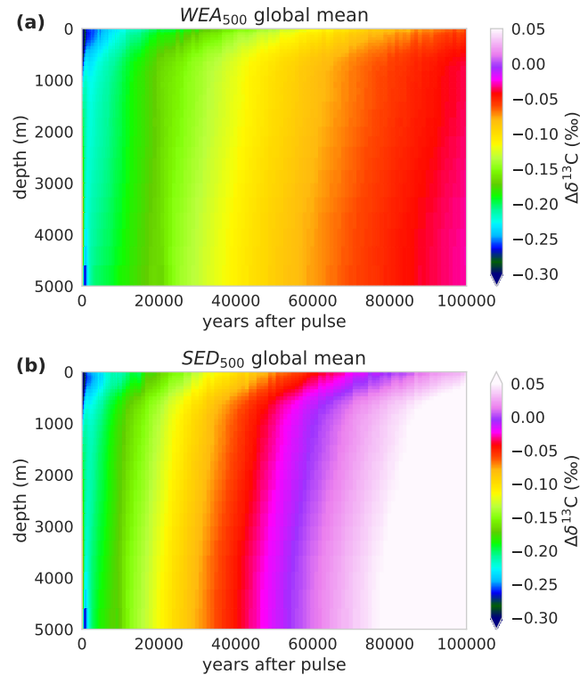
Figure 3: New Fig. A1 for the revised manuscript: Hovmoeller-type diagram showing the temporal evolution of the global-mean vertical profile of \Delta\delta^{13}\text{C}_{DIC} for experiment (a) WEA_{500} and (b) SED_{500} .
