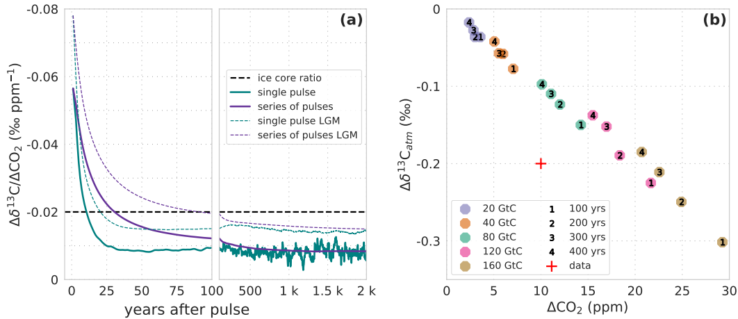
Figure 4: New Fig. 8 for the revised manuscript: (a) Temporal evolution of the ratio of \Delta\delta^{13}\text{C} to \Delta\text{CO}_2 in the atmosphere. Results are from simulations WEA_{100} forced by preindustrial boundary conditions (solid lines) and LGM_{100} forced by Last Glacial Maximum boundary conditions (thin dashed lines). Carbon is released as a single pulse at year 0 (green lines) or assumed to be released at a uniform rate from year 0 to the year plotted (purple lines; see main text). The dashed horizontal line indicates a \Delta\delta^{13}\text{C} to \Delta\text{CO}_2 ratio of -0.2 ‰ to 10 ppm as seen in ice core records for HS1 and HS4. (b) Response in \Delta\text{CO}_2 and \Delta\delta^{13}\text{C}_{\text{atm}} to a uniform release of 20, 40, 80, 120, and 160 GtC (colors) of isotopically light carbon ( \delta^{13}\text{C} = -24 ‰) to the atmosphere over 100, 200, 300, and 400 years (numbers). Shown is the mean over 30 years starting in the last year of the release. Red cross indicates the approx. \Delta\delta^{13}\text{C} to \Delta\text{CO}_2 change as seen in ice core records for HS1 and HS4 (Bauska et al., 2016, 2018).
