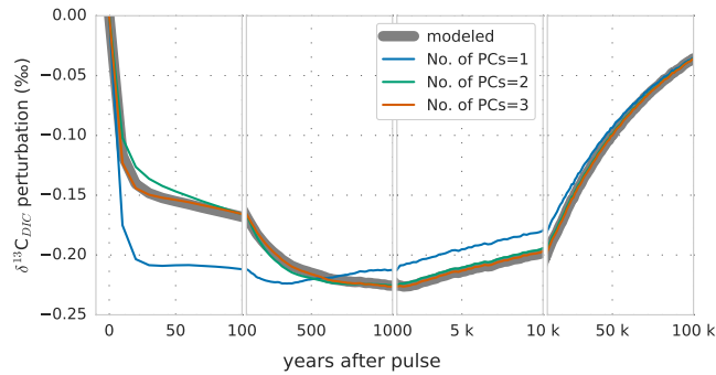
Figure 5. Modeled and reconstructed global-average perturbation of the isotopic signature of dissolved inorganic carbon in the ocean ( \delta^{13}\text{C}_{DIC-DIC} ; thick gray line ) in response to a carbon pulse to the atmosphere of 500 GtC with a \delta^{13}\text{C} signature of -24 ‰. The thin colored lines show the perturbation as reconstructed with one (blue), two (green), and three (orange) principal components for a 500 carbon pulse with \delta^{13}\text{C} = -24 .
