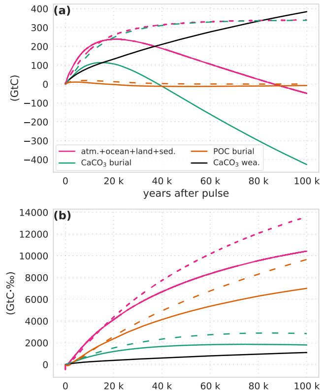
Figure 2: New Fig. 4 for the revised manuscript: The perturbation budget for (a) carbon and (b) carbon isotopes. Solid lines show results from experiment WEA_{500} , dashed lines from experiment SED_{500} . In both panels the pulse (500 GtC, -12,000 GtC·‰) is subtracted from the combined atmosphere-ocean-land-reactive sediment inventory. Burial fluxes are plotted inversely and the sum of burial (green, orange lines) and weathering (black) fluxes yields the combined inventory (pink).
