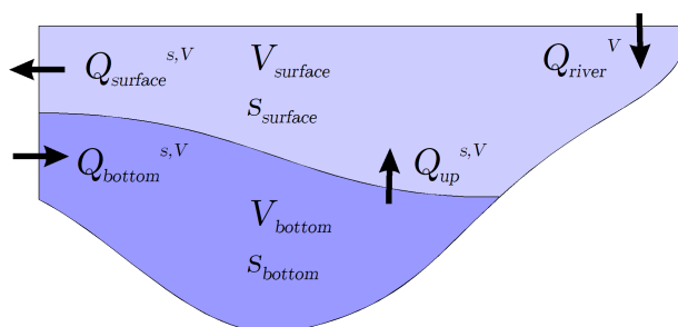
Figure 4. Schematic view of salt and volume fluxes in and out of two compartments, separated by an isohaline. The volumes V and salt masses s inside these compartments change over time.
