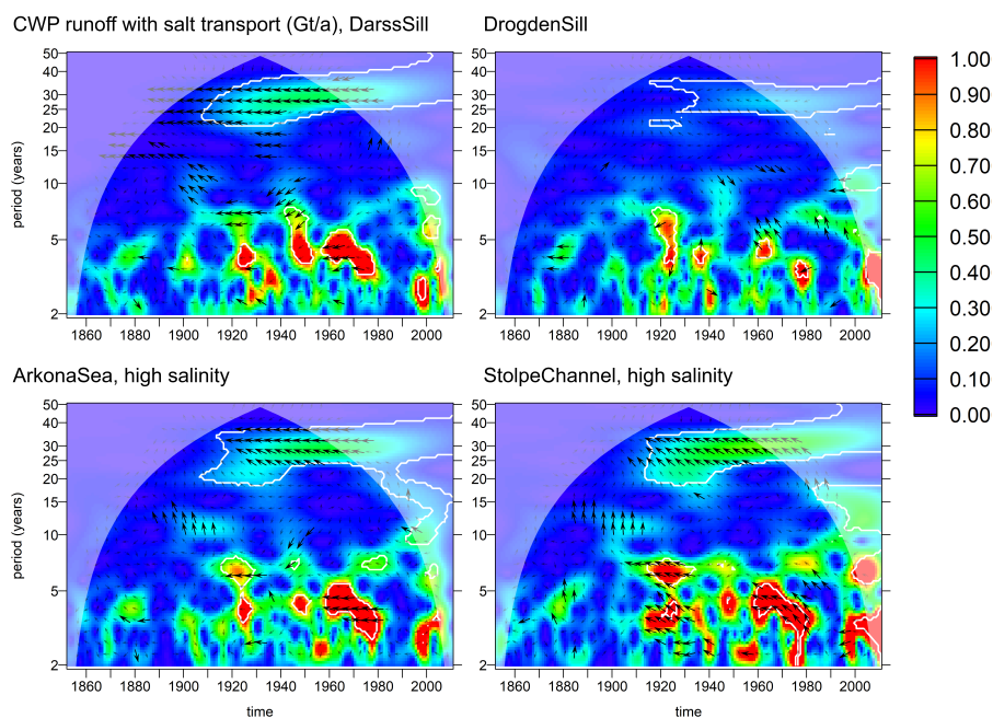
Figure 16. Common wavelet power between salt import across selected transects and normalised annual runoff into the Baltic Sea. T_{\hat{S},t} is chosen as time series for salt import across DarssSill and DrogdenSill transects, while T_{highsal,t} is chosen across ArkonaSea and StolpeChannel. White contours indicate that the WA/CWP is significant at the 95% confidence level with respect to a random shuffling of the annual means of the runoff. Arrows indicate relative phase: \rightarrow =in phase, \downarrow =runoff leading salt import by 90^\circ . Thick arrows indicate phase stability (wavelet coherence > 0.95 ).
