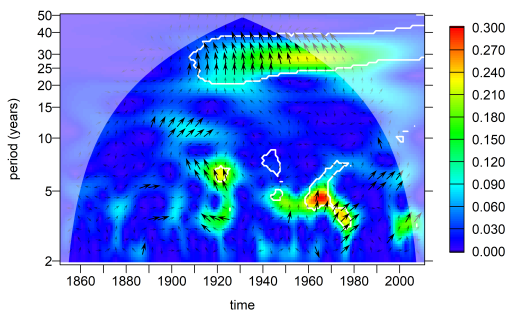
Figure 10. Top row: Wavelet amplitude of the relative deviation in runoff of all model rivers inside the ArkonaSea transect, see Fig. 1. Middle row: Common wavelet power between modelled surface salinity at station BY15 (Eastern Gotland Basin, \text{g kg}^{-1} ) and normalised runoff, note that the scale is doubled from Fig. 9. Bottom row: The same for bottom salinity. White contours indicate that the WA/CWP is significant at the 95% confidence level with respect to a random shuffling of the annual means of the runoff. Arrows indicate relative phase: \rightarrow =high runoff and salinity in phase, \uparrow =low runoff leading salinity by 90^\circ . Thick arrows indicate phase stability (wavelet coherence > 0.95 ).
