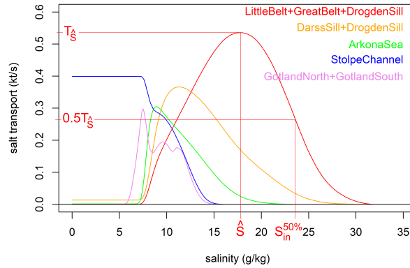
Figure 2. Net salt transports into the Baltic Sea above a specific salinity level, temporal average across the simulation period 1850–2008. Most curves tend to values close to zero at low salinities, indicating that no systematic salt gain or loss occurs inside closed transects. Stolpe Channel and DarssSill+DrogdenSill transects are not closed, the latter due to the existence of the Storstrømmen channel in the model.
