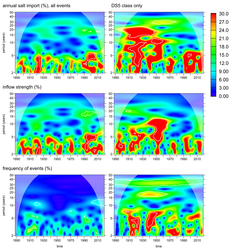
Figure 11. Wavelet analysis of the relative change in inflow activity (%). Top row: total salt import. Middle row: Inflow strength as mean salt import during a single inflow event. Bottom row: Inflow frequency as number of inflows per year.
