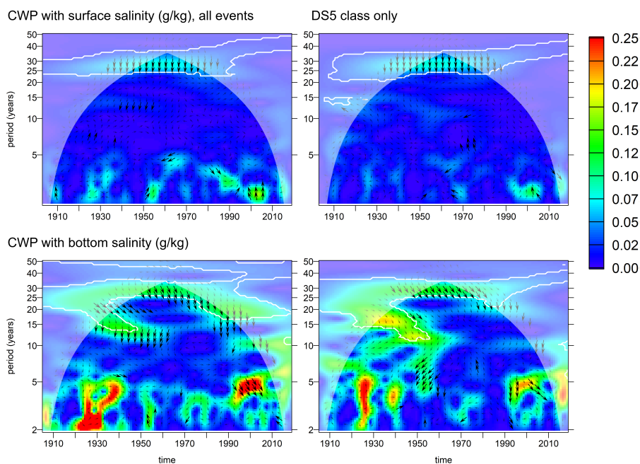
Figure 12. Common wavelet power between observed surface and bottom salinity at station BY15 (Eastern Gotland Basin) and normalised annual import of salt by inflow events. Left column: All inflow events identified in Mohrholz (2018). Right column: Only DS5 class events. White contours indicate that the WA/CWP is significant at the 95% confidence level with respect to a random shuffling of the annual means of the salt import. Arrows indicate relative phase: \rightarrow = in phase, \downarrow =salt import leading salinity by 9^\circ . Thick arrows indicate phase stability (wavelet coherence > 0.95 ). The region where arrows are not drawn indicates the cone of influence for the common wavelet power, the white shading indicates the cone of influence for the wavelet coherence.
