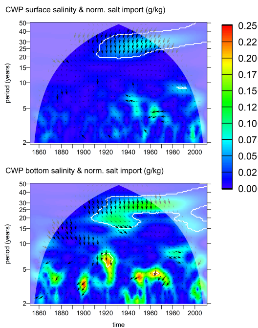
Figure 14. Common wavelet power between modelled surface and bottom salinity at station BY15 (Eastern Gotland Basin) and the normalised time series of T_{S,t} across the transect ArkonaSea ( \text{g kg}^{-1} ). White contours indicate that the WA/CWP is significant at the 95% confidence level with respect to a random shuffling of the annual means of the salt import. Arrows indicate relative phase: \rightarrow =in phase, \perp =salt import leading salinity by 90^\circ . Thick arrows indicate phase stability (wavelet coherence > 0.95 ).
