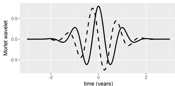
Figure 3. The Morlet wavelet for the temporal scale a = 1 year and \omega_0 = 6 . Solid line: real part. Dashed line: imaginary part. Please note that the periodicity almost matches the temporal scale.
