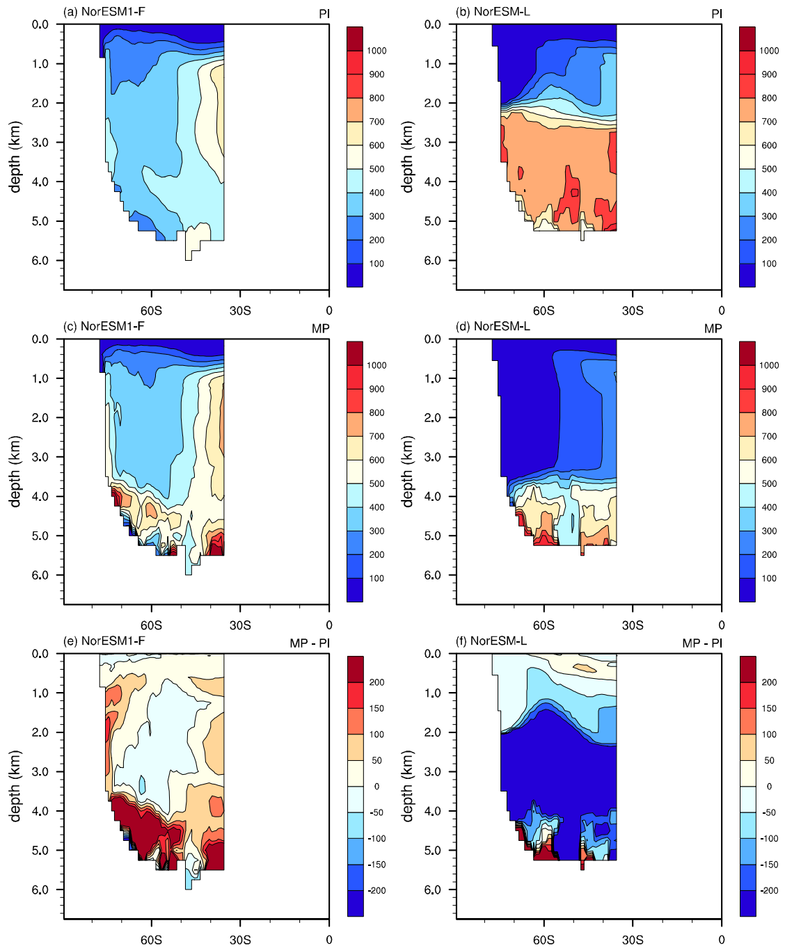
Fig. S1. Climatological Southern Ocean ideal age (units: year) derived from the pre-industrial (a and b) and Pliocene (c and d) experiments, and their differences (e and f) according to NorESM1-F (left panel) and NorESM-L (right panel).
