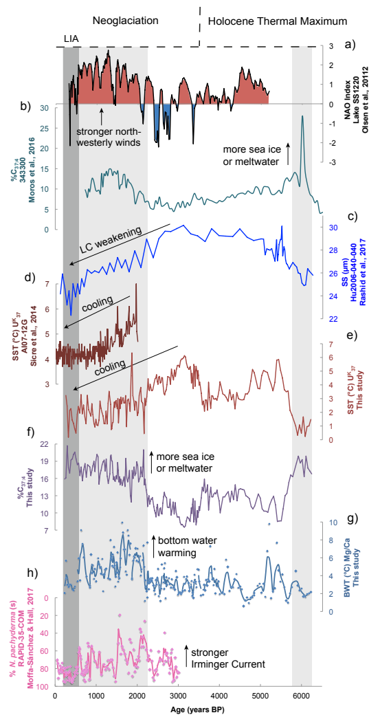
Figure 6: a) The NAO index (Olsen et al., 2012) with positive (red) and negative (blue) phases. b) %C 37:4 in core 343300 (Moros et al., 2016). c) SS mean (µm) in core Hu2006-040-040 (Rashid et al., 2017). d) SST record in Newfoundland core AI07-12G (Siere et al., 2014). e) SST record based on the U 37 K index (this study). f) Higher proportions of %C 37:4 are interpreted to reflect a longer sea ice season or meltwater. g) BWT estimates are based on Mg/Ca ratios in benthic foraminifera N. labradorica and reflect subsurface conditions. h) Lower abundances of polar water planktic foraminifera species N. pachyderma in central Labrador Sea core RAPiD-35-COM indicate warming due to stronger IC inflow (Moffa-Sánchez and Hall, 2017).
