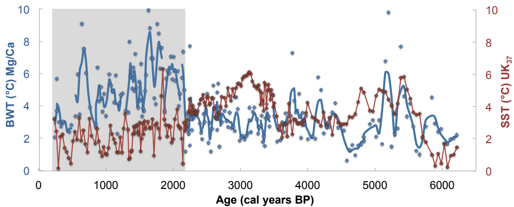
Figure 5: Surface (red) and bottom (blue) water temperature reconstructions are based on the alkenone U_{37}^K index and Mg/Ca ratios of benthic foraminifera N. labradorica , respectively. In contrast to the surface record, the BWT record is displayed with a 3-point-running mean due to the 2°C uncertainty of individual data points. Both records show a similar temperature range 5 between 6.1 and 2.1 ka BP. After 2.1 ka BP, the BWT record displays higher fluctuations and a shift to warmer average temperatures, leading to a temperature reversal in the water column with generally warmer bottom waters underlying colder surface waters in this interval. The warming of bottom waters is associated with a stronger inflow of the westward retroflection of the WGC reaching our core site at 566m depth underneath the cold inner LC.
