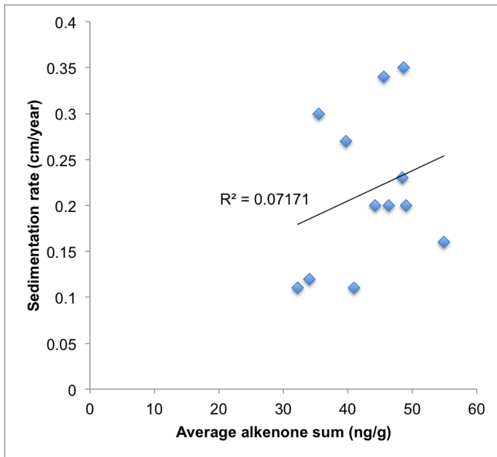
Fig. 2. Relationship of alkenone sum and sedimentation rate
