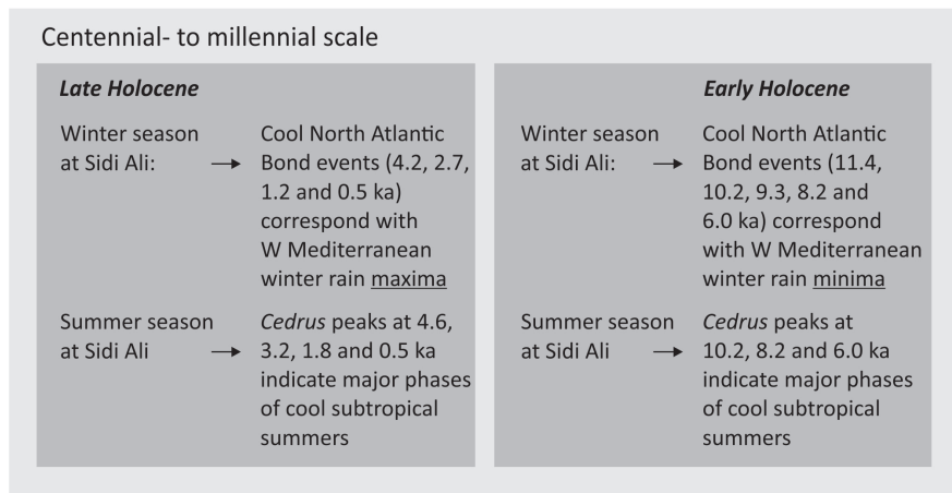
Fig. 1. Lake Sidi Ali Holocene core: illustration of major conclusions
