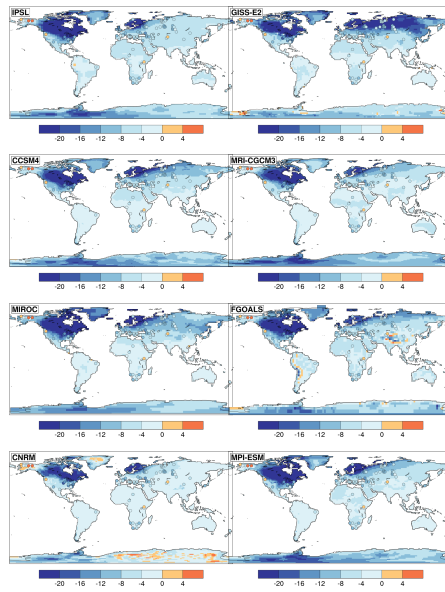
Figure 7: Background color fill: simulated global pattern of annual mean surface temperature over land ( T_{s,s} ) (in ^{\circ}\text{C} ) changes between the eight PMIP3 model and PI climate. The circles localize the pollen-based reconstructed temperature changes by Bartlein et al. (2011).
