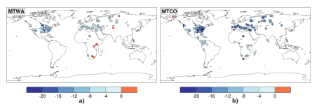
Fig. S3: Reconstructed anomalies (in °C) between LGM and P1 of mean temperature of the warmest month (MTWA) (a) and mean temperature of the coldest month (MTCO) (b) by Bartlein et al. (2011).
