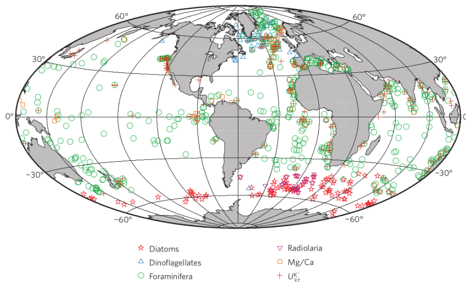
Fig. 1. Fig. S1: Distribution of MARGO data points, indicating also which proxy was measured at each location (Waelbroeck et al., 2009 ©Nature Geoscience).
