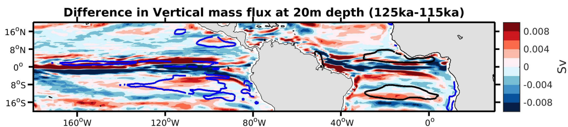
Figure R3: Difference in Vertical volume flux (positive depicts upward) between 125ka and 115ka. The blue (black) lines depict a decrease (increase) by -4 \text{ g C m}^{-2} \text{ yr}^{-1} .
