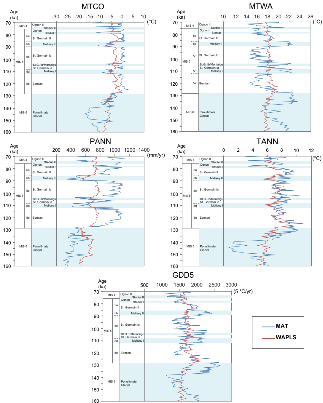
Fig. A Climate reconstruction inferred from Lake Ohrid pollen data, Pinus included. Climate parameters obtained with the MAT method (blue line) and the WAPLS method (red line): MTCO (mean temperature of the coldest month), MTWA (mean temperature of the warmest month), PANN (mean annual precipitation), TANN (mean annual temperature) and GDD5 (growing degrees days over 5° C). Climate parameter values are plotted against age (ka); this figure can be compared with Fig. 2 (climate reconstruction, Pinus excluded)
