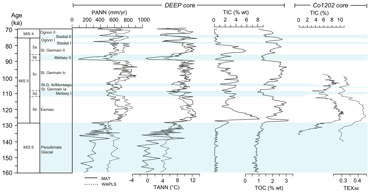
Fig. 4 Lake Ohrid: Comparison between DEEP core annual temperature (TANN), precipitations (PANN) and TIC (Francke et al., 2016) with TIC and TEX 86 (Co1202 core, Holtvoeth et al., 2017). Blue shading indicates cold periods ( Riss penultimate glacial and early Würm last glacial stadials).
