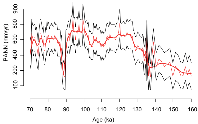
Fig. BA MAT and WAPLS error bars for PANN and TANN climate parameters. The last graph represents the squared-chord distance between the first and the last analogue for a chosen climate parameter (TANN) calculated by MAT method.
