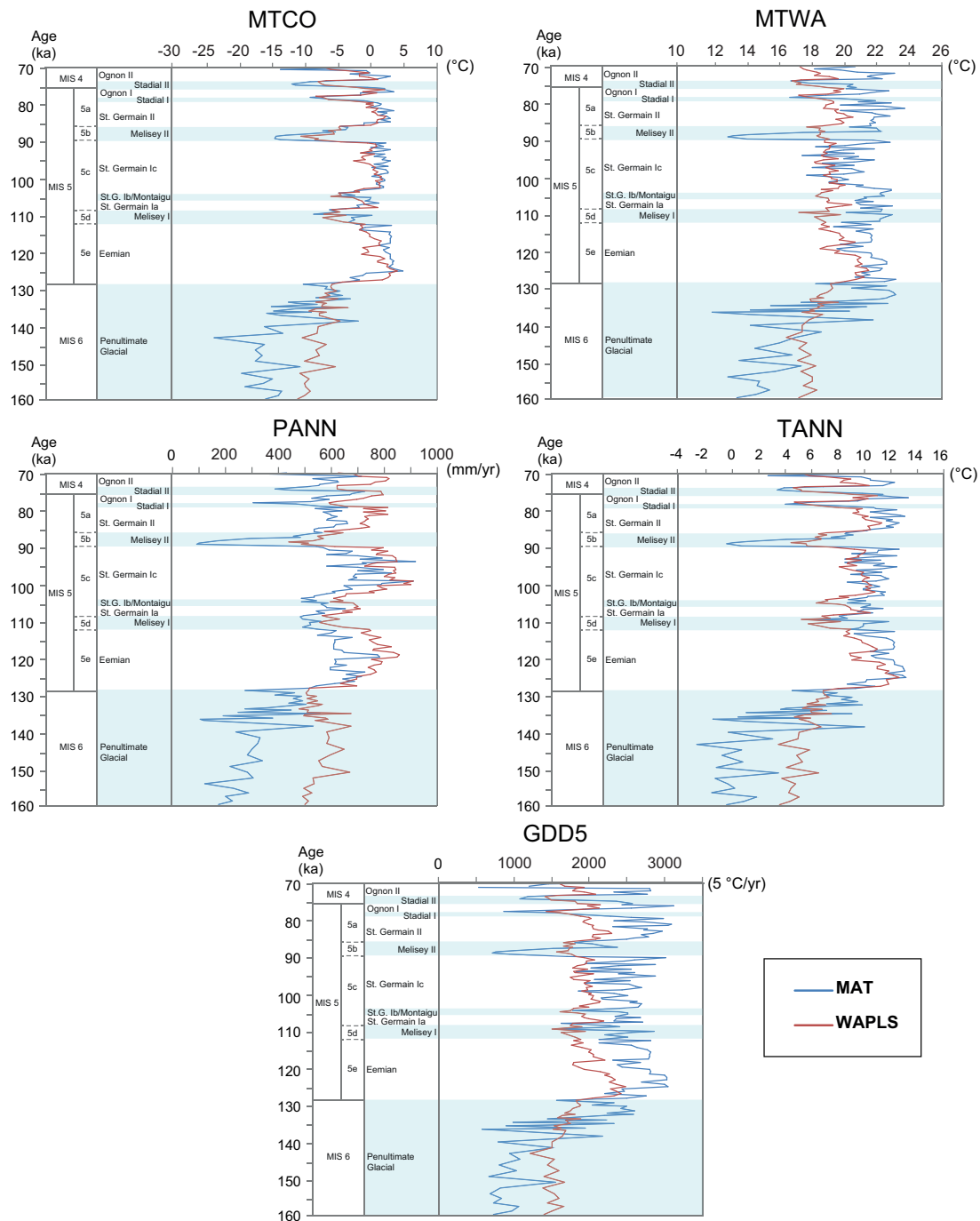
5 Fig. 3 Climate reconstruction inferred from Lake Ohrid pollen data (Sadori et al., 2016; Sinopoli et al., 2018). Climate parameters obtained with the MAT method (black-blue line) and the WAPLS method (red line): MTCO (mean temperature of the coldest month), MTWA (mean temperature of the warmest month), PANN (mean annual precipitation), TANN (mean annual temperature) and GDD5 (growing degrees days over 5° C). Climate parameter values are plotted against age (ka); they are not expressed in anomalies (past climate value minus the modern measured value). Blue shading indicates cold periods ( Riss penultimate glacial and Early-early Würm last glacial stadials). Blue shading indicates cold periods (Riss glacial and Early Würmian glacial stadials).
