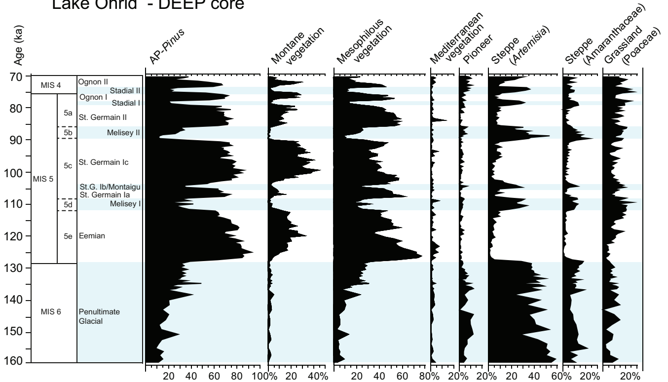
Fig. 2 Lake Ohrid (FYROM/ Albania) - DEEP core - Pollen percentage diagram of selected taxa and ecological groups, against age (ka). Montane vegetation+rees : Abies , Betula , Fagus , Ilex , Picea ; mesophilous vegetation+rees : Acer , Buxus , Carpinus betulus , Castanea , Celtis , Corylus , Fraxinus excelsior/oxycarpa , Ostrya/Carpinus orientalis , Hedera , Quercus robur type, Quercus cerris type, Tilia , Ulmus , Zelkova ; mediterranean vegetation+rees : Cistus , Fraxinus ornus , Olea , Phillyrea , Pistacia , Quercus ilex type, Rhamnus ; steppe: Artemisia , Amaranthaceae , Chicoriodeae and Asteroideae and grassland: Poaceae and Cyperaceae . Data from Sadori et al. (2016) and Sinopoli et al. (2018).
