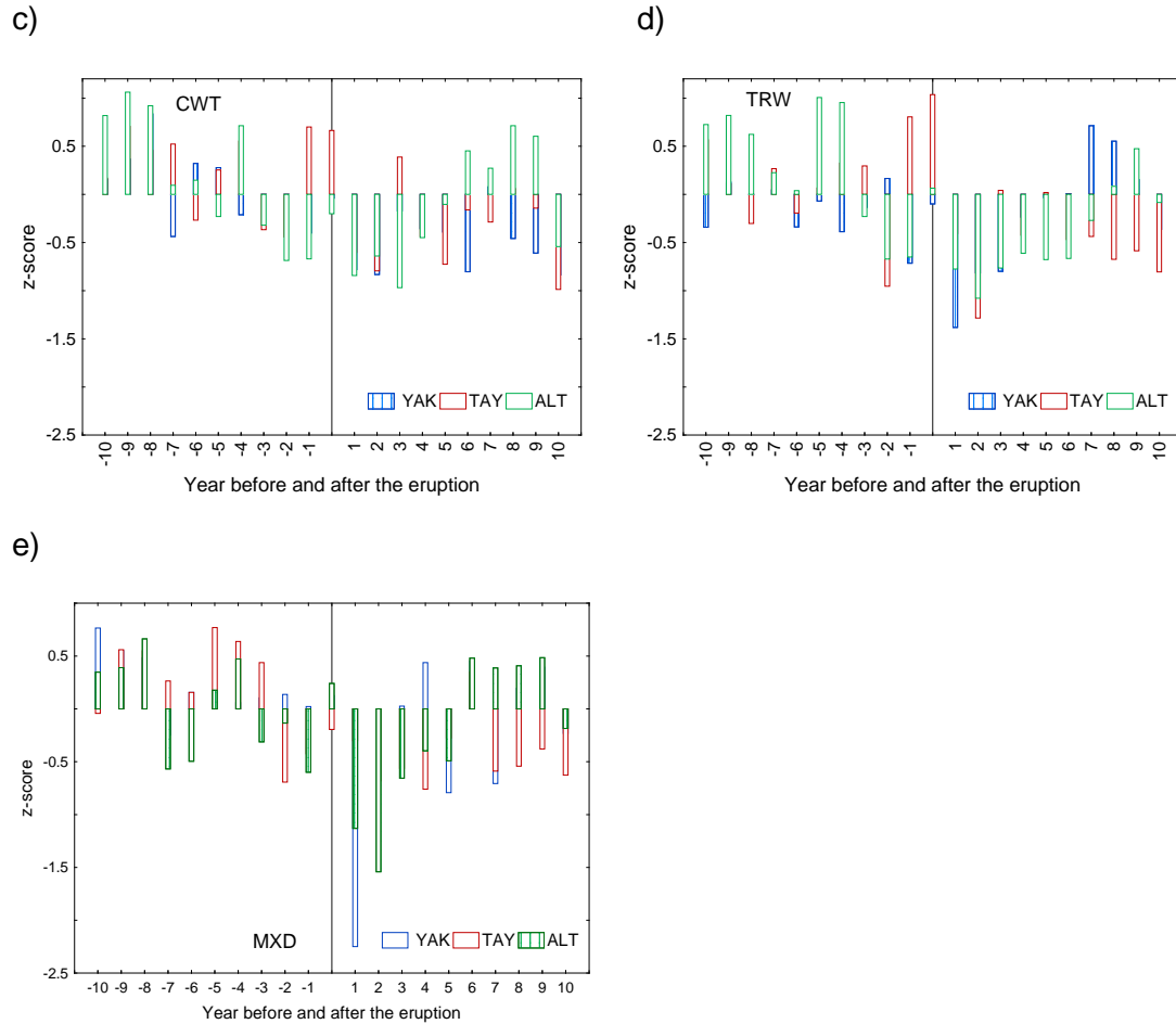
Fig. 3. Superposed epoch analysis of \delta^{18}\text{O} (a), \delta^{13}\text{C} (b), CWT (c), TRW (d) and MXD (e) chronologies for each study site and for the major volcanic eruptions in CE 535, 1257, 1641, 1815 and 1991.
