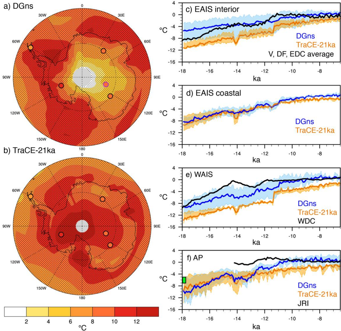
Figure 2: Surface temperature change ( ^{\circ}\text{C} ) as simulated in (a) \text{DG}_{\text{ns}} and (b) TraCE-21ka for the period of 18 to 6.5 ka. Ice core locations of the JRI, WDC, DF, V, and EDC sites are marked by filled circles, with the fill color corresponding to the change estimated in the ice core record, black outlines indicating a match in warming between the ice core and model simulation (i.e., the ice core temperature change from 18 to 6.5 ka is within the range of seasonal temperature changes of the climate model), and green (purple) outlines indicating an overestimation (underestimation) in warming by the models. For these model-proxy comparisons, we use site-specific model averages of land surface grid cells: JRI ( 63\text{--}65^{\circ}\text{S} , 59\text{--}62^{\circ}\text{W} ), WDC ( 77\text{--}82^{\circ}\text{S} , 115\text{--}109^{\circ}\text{W} ), DF ( 75\text{--}79^{\circ}\text{S} , 36\text{--}42^{\circ}\text{E} ), V ( 77\text{--}82^{\circ}\text{S} , 104\text{--}110^{\circ}\text{E} ), EDC ( 73\text{--}77^{\circ}\text{S} , 121\text{--}127^{\circ}\text{E} ). Stippling indicates a difference between decadal output of 18.0-17.5 ka and 7.0-6.5 ka that is significant at the 95% confidence level. (c-e) 100-yr average surface temperature time series ( ^{\circ}\text{C} ) of four regions (EAIS interior: 83^{\circ}\text{S}\text{--}75^{\circ}\text{S} , 30^{\circ}\text{W}\text{--}165^{\circ}\text{E} ; coastal EAIS: 75^{\circ}\text{S}\text{--}68^{\circ}\text{S} , 15^{\circ}\text{W}\text{--}165^{\circ}\text{E} ; WAIS: 83^{\circ}\text{S}\text{--}72^{\circ}\text{S} , 165^{\circ}\text{E}\text{--}30^{\circ}\text{W} ; AP: 72^{\circ}\text{S}\text{--}64^{\circ}\text{S} , 64^{\circ}\text{W}\text{--}59^{\circ}\text{W} ) relative to PI of both model simulations and ice core temperature reconstructions of sites located therein ( \text{DG}_{\text{ns}} in blue, TraCE-21ka in orange, ice cores in black). The colored shading indicates the seasonal range calculated from the 100-yr average austral summer and winter temperature anomalies. For EAIS, the ice core reconstruction is an
