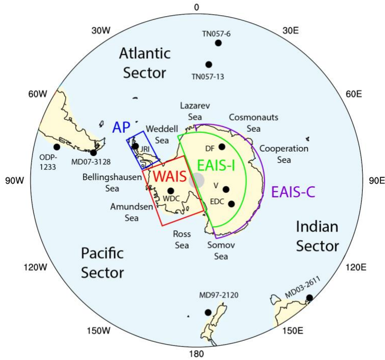
1060 Figure 1: Polar-stereographic view of Antarctica and the Southern Ocean (maximum Latitude of 35°S). The 1065 colors indicate the land and ocean mask of the TraCE-21ka simulation (yellow and light blue, respectively). The continental regions, namely, the Antarctic Peninsula (AP), the West Antarctic Ice Sheet (WAIS), the East Antarctic Ice Sheet interior (EAIS-I), and the East Antarctic Ice Sheet coastal region (EAIS-C) are outlined in the colored boxes (blue, red, green, and purple, respectively). The locations of the Antarctic ice core and marine sediment records used in this analysis are indicated by the black dots.
