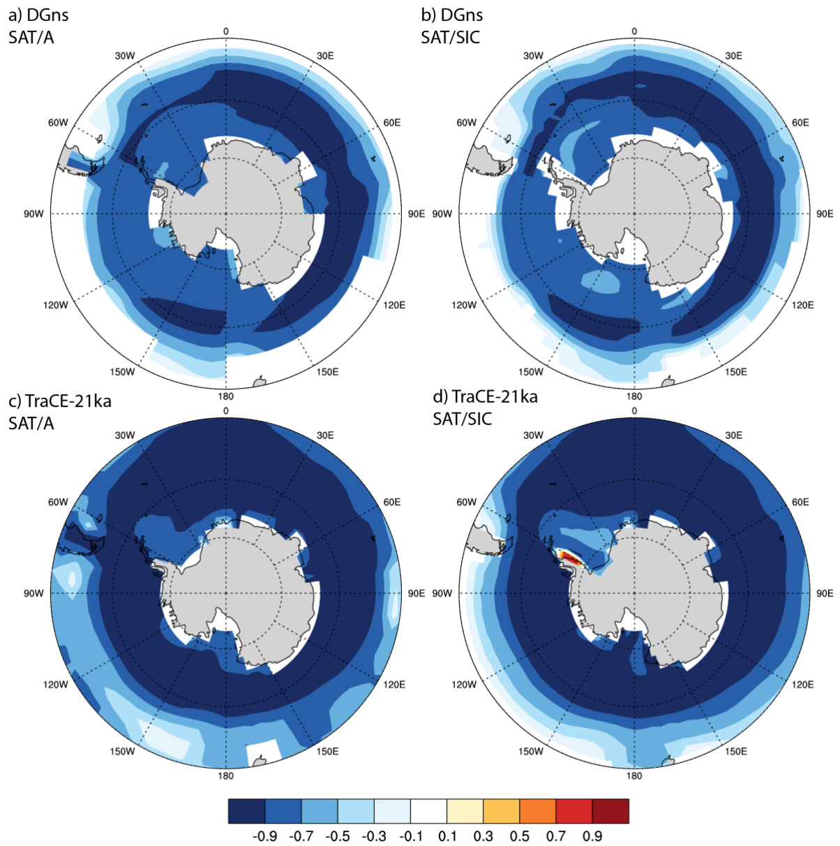
1155 Figure 11: Spatial Pearson linear cross-correlation coefficients ( r ) between decadal surface air temperature (SAT, °C), surface albedo (A), and sea ice coverage (SIC, %) for (a-b) DG ns and (c-d) TraCE-21ka. DG ns SAT was regridded to the same grid as DG ns SIC using bilinear interpolation in panel b.
