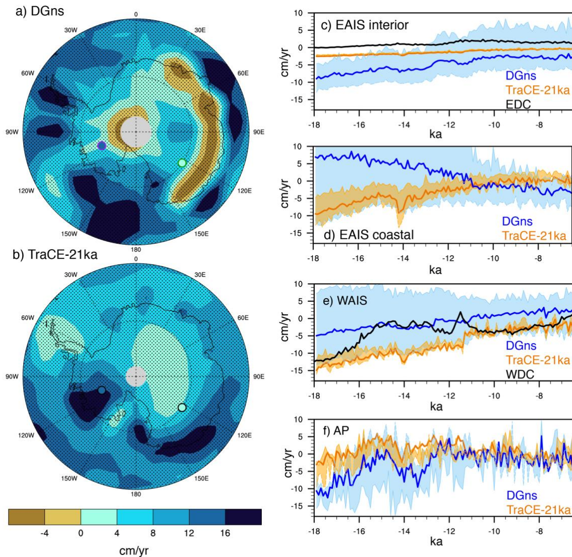
Figure 3: Precipitation change (cm/yr) as simulated in (a) DG_{ns} and (b) TraCE-21ka for the period of 18 to 6.5 ka. Ice core locations of WDC and EDC are marked by filled circles, with the fill color corresponding to the change estimated in the ice core record, black outlines indicating a match in warming between the ice core and model simulation (i.e., the ice core temperature change from 18 to 6.5 ka is within the range of seasonal temperature changes of the climate model), and green (purple) outlines indicating an overestimation (underestimation) in warming by the models. For these model-proxy comparisons, we use site-specific model averages of land surface grid cells: WDC ( 77\text{-}82^\circ\text{S} , 115\text{-}109^\circ\text{W} ), EDC ( 73\text{-}77^\circ\text{S} , 121\text{-}127^\circ\text{E} ). Stippling indicates a difference between decadal output of 18.0-17.5 ka and 7.0-6.5 ka that is significant at the 95% confidence level. (c-f) 100-yr average accumulation time series (cm/yr) of four regions (EAIS interior: 83^\circ\text{S}\text{-}75^\circ\text{S} , 30^\circ\text{W}\text{-}165^\circ\text{E} ; coastal EAIS: 75^\circ\text{S}\text{-}68^\circ\text{S} , 15^\circ\text{W}\text{-}165^\circ\text{E} ; WAIS: 83^\circ\text{S}\text{-}72^\circ\text{S} , 165^\circ\text{E}\text{-}30^\circ\text{W} ; AP: 72^\circ\text{S}\text{-}64^\circ\text{S} ,
