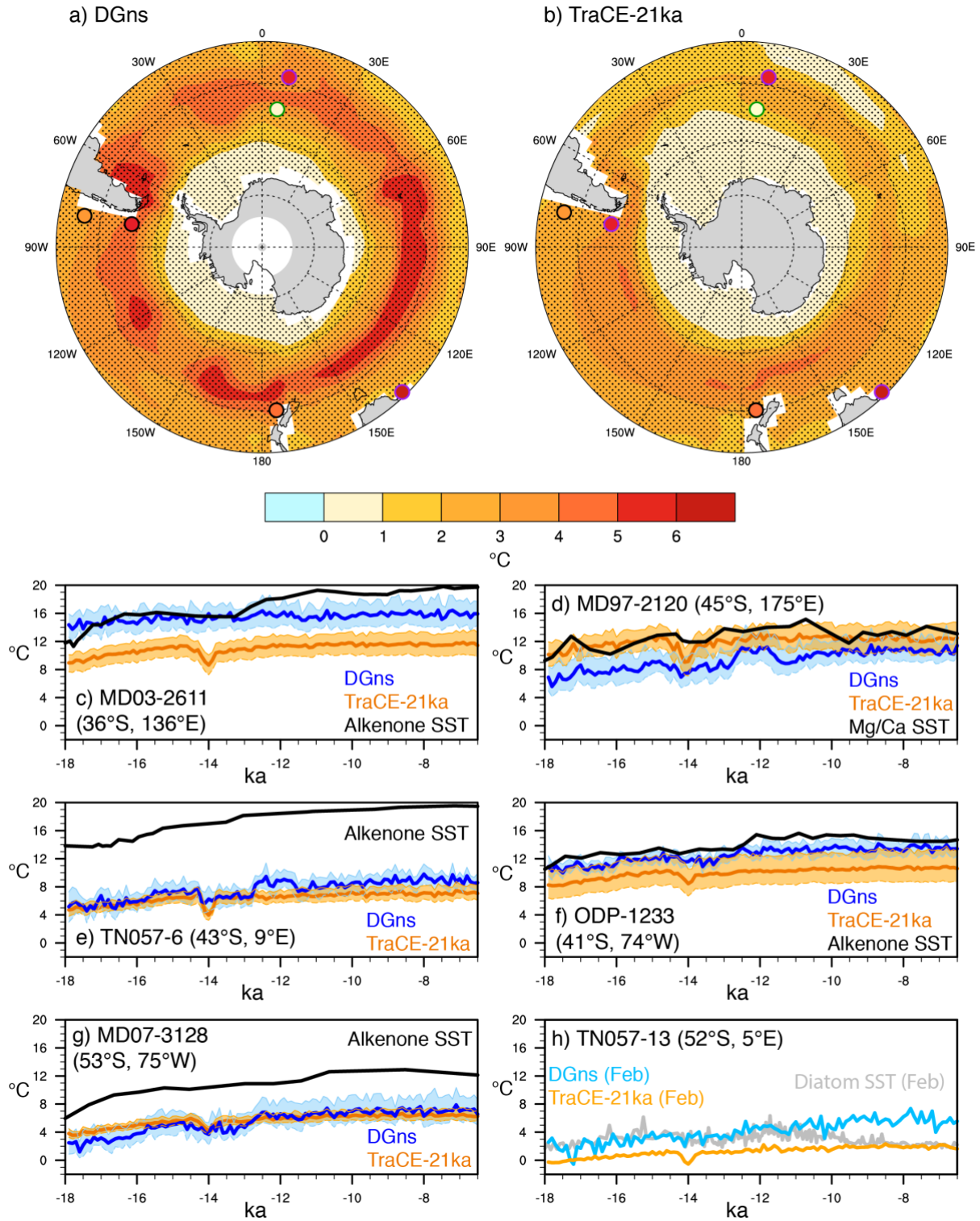
Figure 6: Sea surface temperature (SST) change (°C) as simulated in (a) DG ns and (b) TraCE-21ka for the period of 18 to 6.5 ka. Marine sediment locations are marked by open circles, with black outlines indicating a match in warming between the ice core and model simulation (i.e., the estimated proxy SST change from 18 to 6.5 ka is within the range of seasonal SST changes of the climate model), and green (purple) outlines indicating an overestimation (underestimation) in warming by the models. Stippling indicates a difference between decadal output of 18.0-17.5 ka and 7.0-6.5 ka that is significant at the 95% confidence level. (c-h) Time series of 100-yr average mean annual SST from the models and SST proxy reconstructions (°C) at each individual marine
