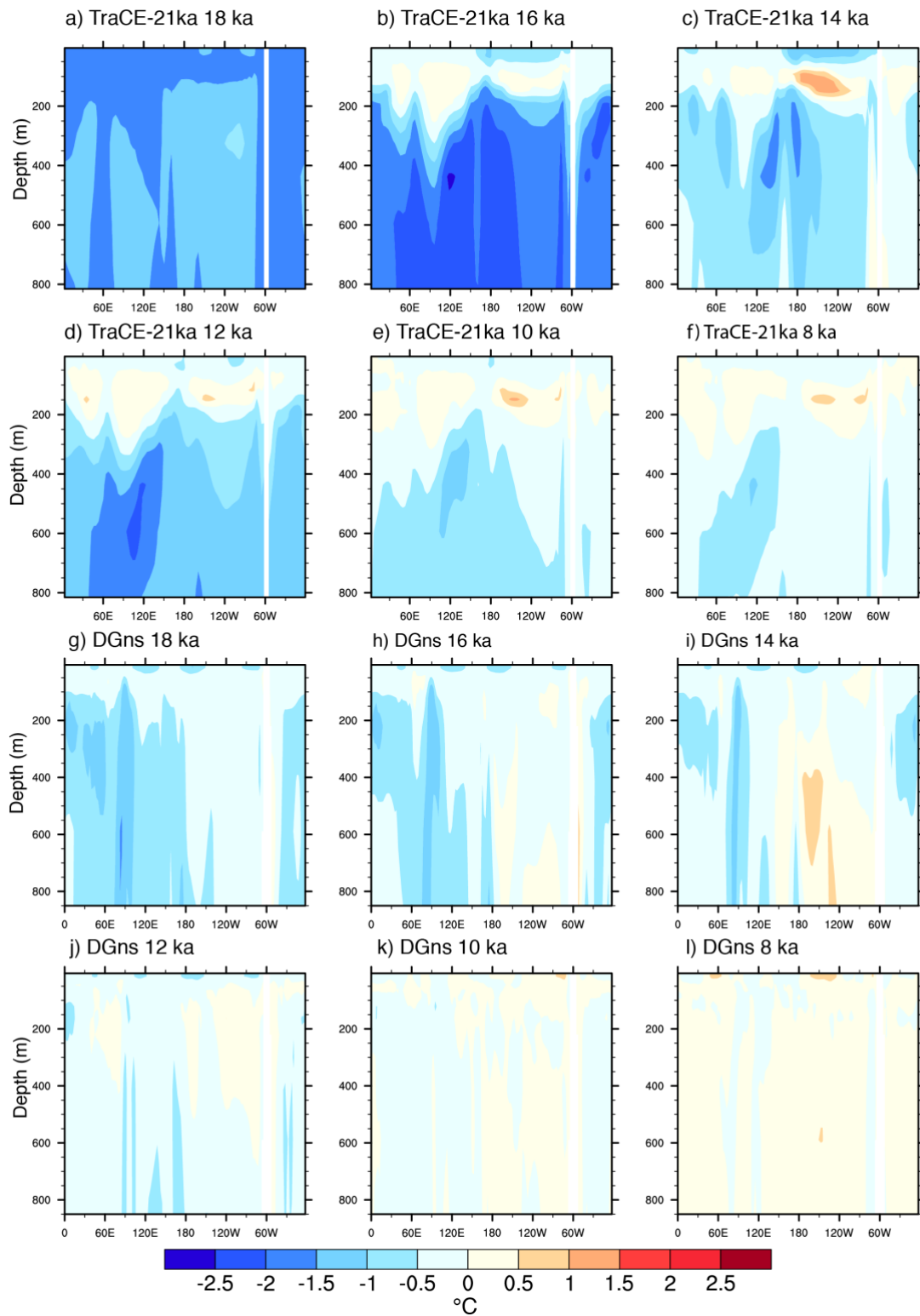
1135 Figure 8: 2-ka time slices of longitudinal cross-sections of 100 yr-averaged ocean temperature anomalies relative to PI at 64°S the surface to 800 m depth: (a-f) TraCE-21ka 18ka to 8 ka; (g-l) DG ns 18ka to 8ka.
