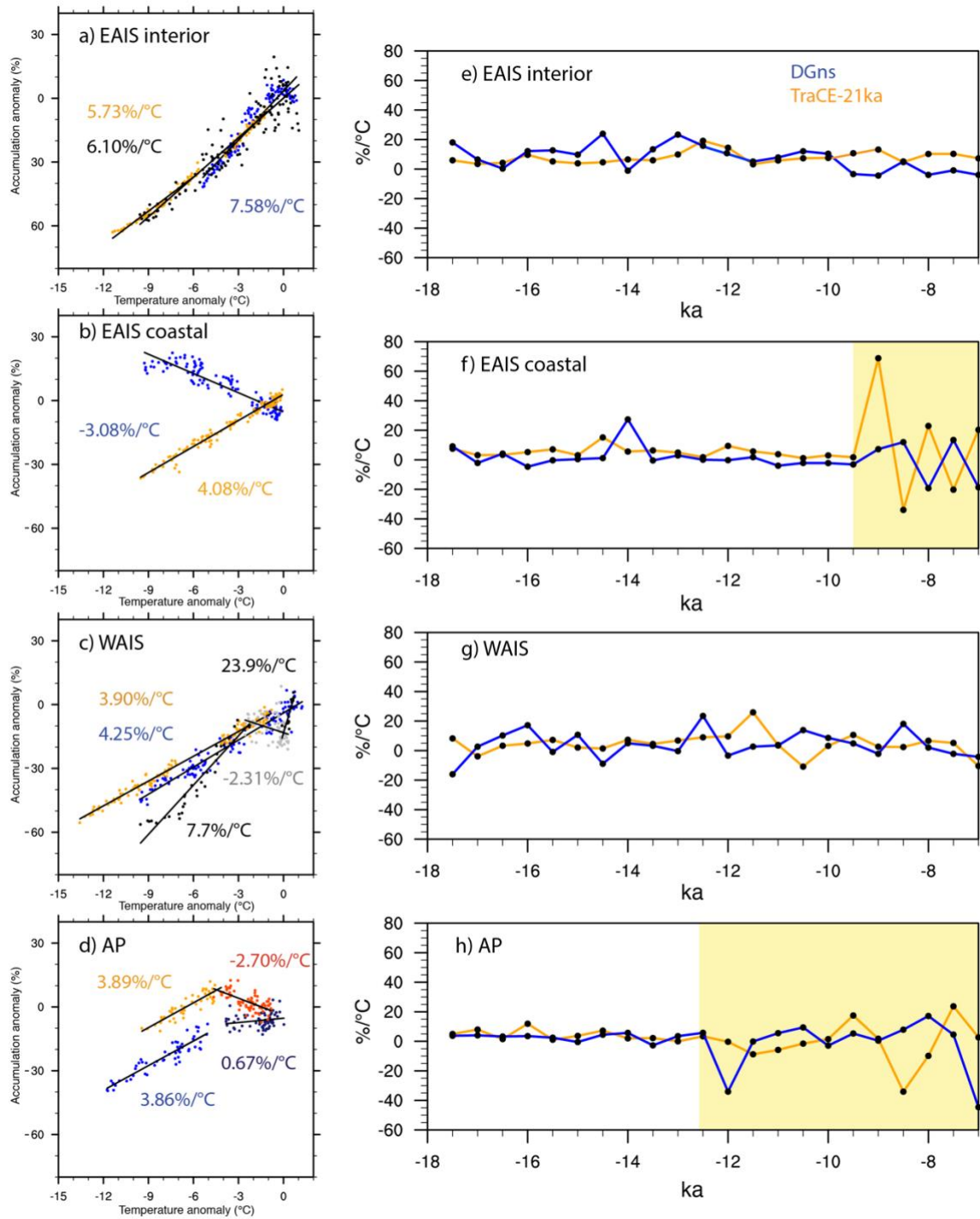
1105 Figure 5: (a-d) Scaling relationships of accumulation (% relative to PI) and temperature (°C relative to PI) in each region. Black and grey dots refer to the proxy record, blue and purple dots refer to the DG NS simulation, and orange and red dots refer to the TraCE21ka simulation. (e-h) The ratio of the change in precipitation (%) to the change in temperature (°C) per 500 years. The yellow bars in panel f and h indicate a shift to higher variability in accumulation-temperature scaling in the AP and EAIS coastal regions.
