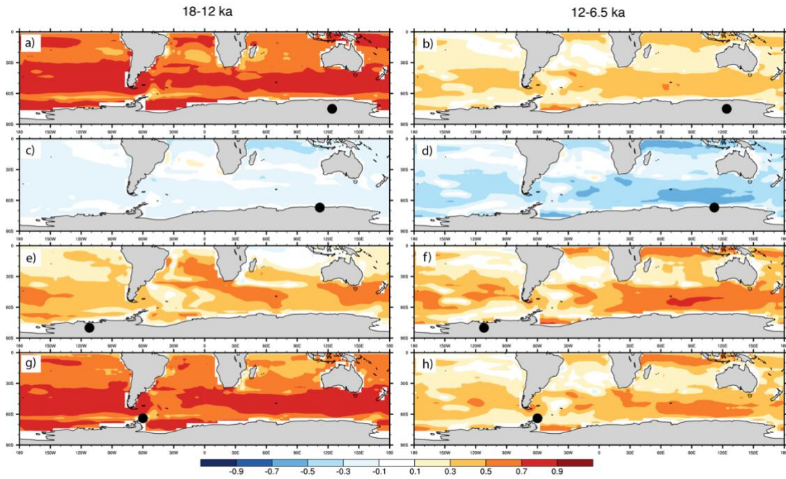
1160 Figure 12: Spatial Pearson linear cross-correlation coefficients ( r ) between decadal SST and precipitation of the 1165 DG_{ns} simulation for (left) 18-12 ka and (right) 12-6.5 ka at the (a,b) EDC (73-77°S, 121-127°E), (c,d) LD (65- 1170 70°S, 110-116°E), (e,f) WDC (77-82°S, 115-109°W), and (g,h) JRI (63-65°S, 59-62°W) ice core locations, respectively.
