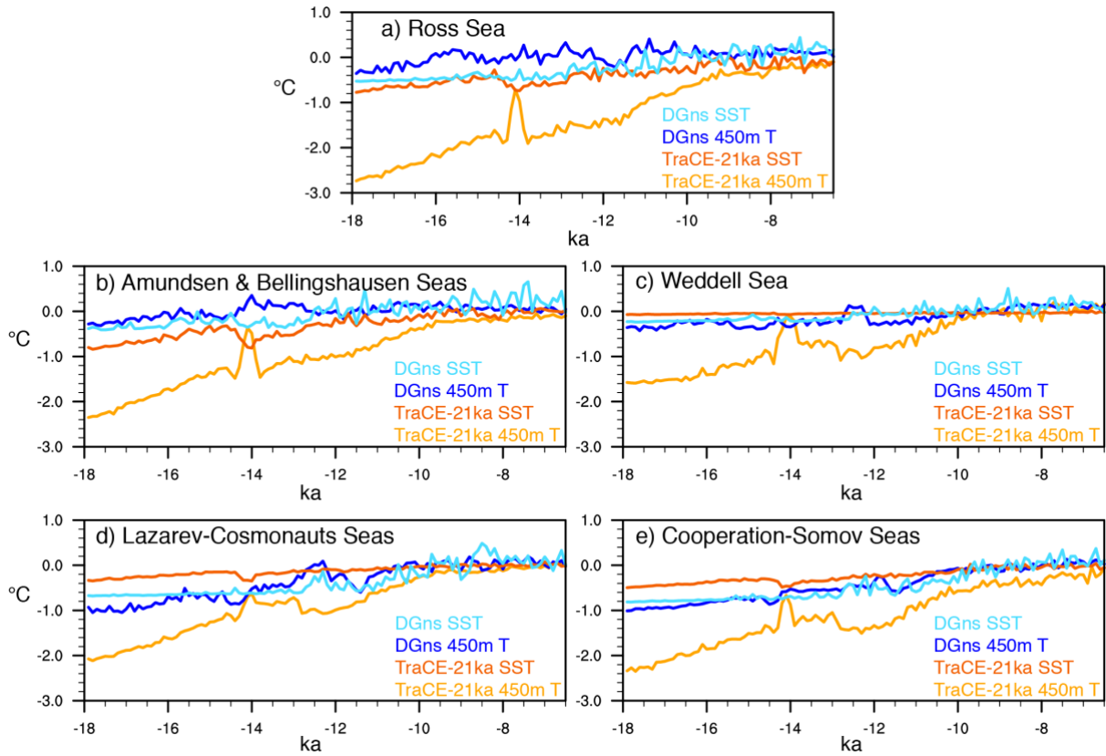
1125 Figure 7: Time series of 100-yr mean annual average SST and 450 m depth ocean temperature anomalies relative to the Preindustrial era (°C) of the coastal seas around Antarctica, namely, (a) the Ross Sea (70°S—62°S, 168°E—160°W), (b) the Amundsen and Bellingshausen Seas (68°S—62°S, 135°W—60°W), (c) the Weddell Sea (70°S—62°S, 60°W—30°W), (d) the coastal region from Lazarev Sea to Cosmonauts Seas 1130 (67°S—62°S, 15°W—50°E), and (e) the coastal region from Cooperation Sea to Somov Sea (67°S—62°S, 55°E—165°E).
