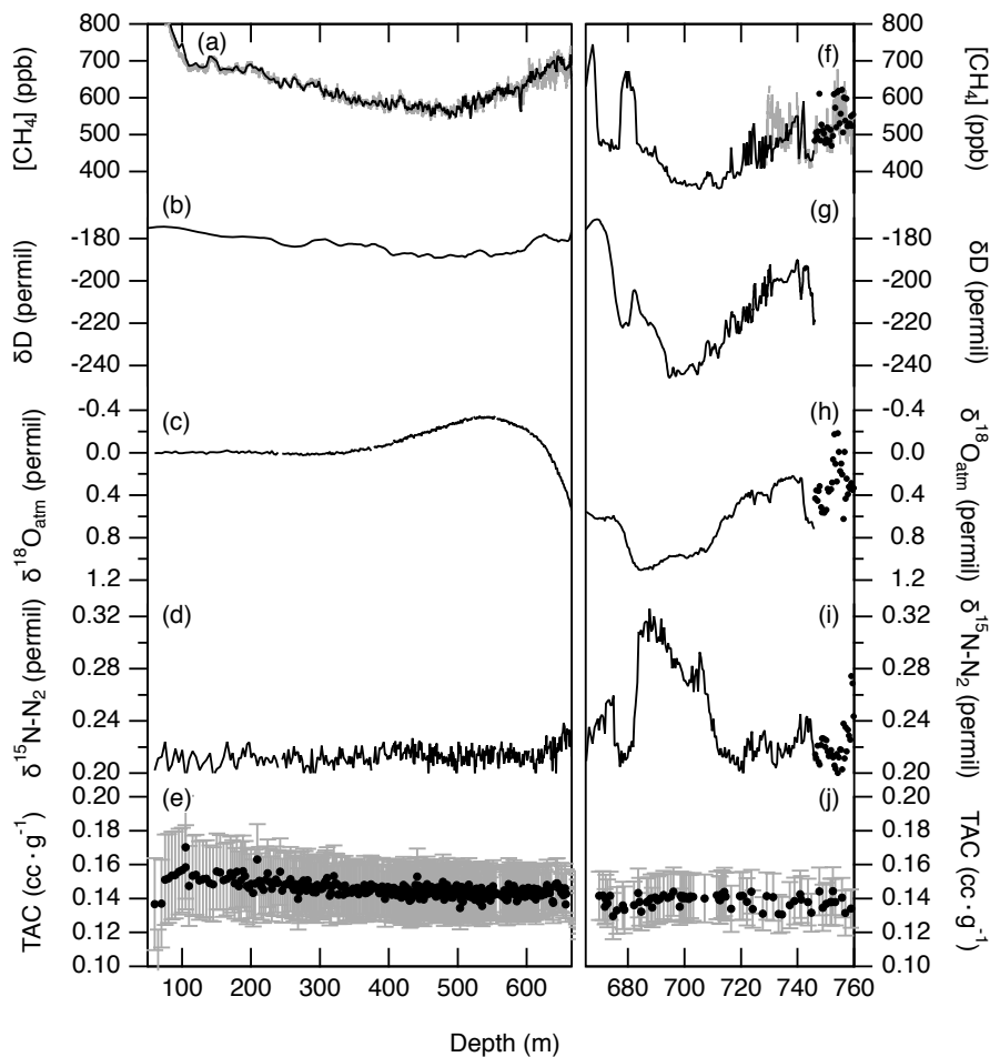
Figure 2. Data from the RICE ice core. Left panel (a-e) (60-665 m) covers the last 11.26 ka; Right panel (f-j) (665-760 m) covers measurements from 11.26-83 ka and measurements from the 9 m of ice below the dated section. (a, f) Continuous methane measurements, gray, between 0-726 m depth are calibrated to discrete methane measurements, black. Beyond 726 m depth, raw CFA methane measurements are plotted. (b, g) Continuously measured \delta\text{D} smoothed with a 500-yr LOESS filter and sub-sampled at 50-yr spacing. (c, h) \delta^{18}\text{O}_{\text{atm}} measurements are corrected for gravitational enrichment in the firn layer using \delta^{15}\text{N}-\text{N}_2 (d, i). (e, j) Total air content (TAC) was measured in conjunction with discrete methane.
