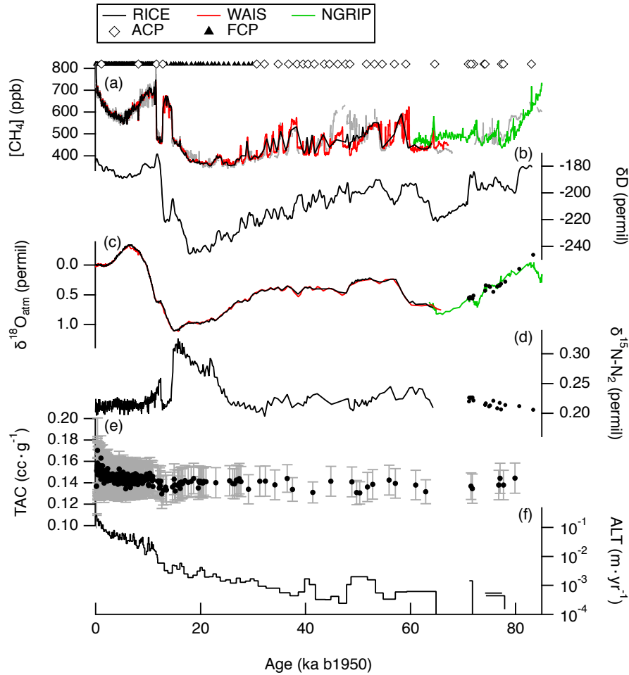
Figure 3. Data from the RICE ice core plotted on the RICE17 age scale. (a) RICE methane and (c) \delta^{18}\text{O}_{\text{atm}} records (gray) shown in comparison to target records from the WAIS Divide ice core on the WD2014 age scale (Buizert et al., 2015b) (red) and NGRIP ice core (Baumgartner et al., 2014; Landais et al., 2007) on a modified GICC05modelext chronology (Wolff et al., 2010) (green). Solid triangles above panel (a) are gas age constraints from a Monte Carlo analysis, open diamonds are prior ACPs from visual matching (see text). (b) \delta\text{D} and (d) \delta^{15}\text{N-N}_2 used in a firm densification model to estimate the ice age-gas age offset. (e) RICE TAC measurements. (f) Mean annual layer thickness calculated from gas age control points adjusted for \Delta\text{age} .
