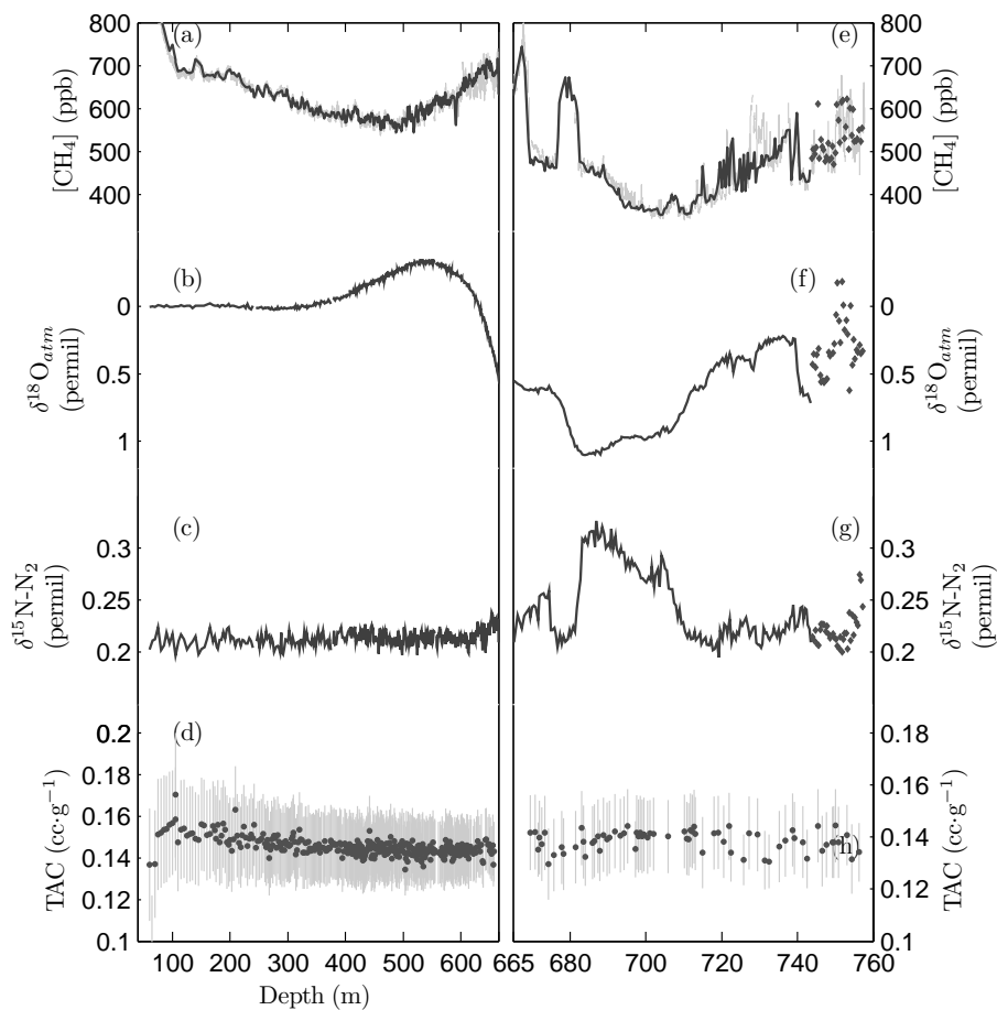
Figure 2. Gas data from the RICE ice core. Left panel (a-d) (60-665 m) covers the last 11.26 ka; Right panel (e-h) (665-760 m) covers measurements from 11.26-83 ka and measurements from the 9 m of ice below the dated section. (a, e) Continuous methane measurements, gray, between 0-726 m depth are calibrated to discrete methane measurements, black. Beyond 726 m depth, raw CFA methane measurements are plotted. (b, f) \delta^{18}\text{O}_{atm} measurements are corrected for gravitational enrichment in the firn layer using \delta^{15}\text{N-N}_2 (c, g). (d, h) Total air content (TAC) was measured in conjunction with discrete methane.
