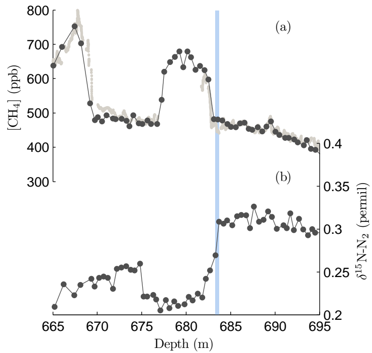
Figure 9. Comparison of (a) methane and (b) \delta^{15}N-N_2 from the RICE ice core plotted on depth. Vertical blue bar highlights the onset of a large decrease in \delta^{15}N-N_2 .
