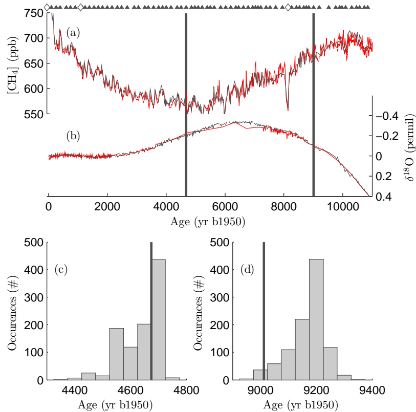
Figure 5. (a) RICE methane and (b) \delta^{18}O_{atm} records matched to those from the WAIS Divide ice core (Rhodes et al., 2015; Buizert et al., 2015b) (red lines) for the last 11.7 ka. FCPs from Monte Carlo routine are shown as solid triangles, prior constraints are shown as open diamonds. Lower panels (c, d) show the distribution of the gas ages for two particular depths, 459.05 m (4675 yr BP) (c) and 621.28 m (9012 yr BP) (d), resulting from the Monte Carlo analysis. The final age of these depths, resulting from the best realization, are shown as vertical gray lines.
