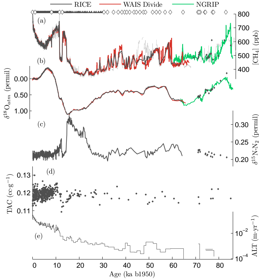
Figure 3. Gas data from the RICE ice core plotted on the RICE17 age scale. (a) RICE methane and (b) \delta^{18}\text{O}_{atm} records (gray) shown in comparison to target records from the WAIS Divide ice core on the WD2014 age scale (Buizert et al., 2015b) (red) and NGRIP ice core (Baumgartner et al., 2014; Landais et al., 2007) on a modified GICC05modelext chronology (Wolff et al., 2010) (green). Solid triangles above panel (a) are gas age constraints from a Monte Carlo analysis, open diamonds are prior ACPs from visual matching (see text). (c) \delta^{15}\text{N-N}_2 is used in a firn densification model to estimate the ice age-gas age offset. (d) RICE TAC measurements. (e) Mean annual layer thickness calculated from gas age control points adjusted for \Delta\text{age} .
