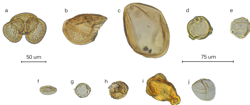
Figure 4. (A) Bar charts showing the relative pollen abundance in each portion of the section (error bars = 95% confidence intervals; MASL- Meters Above Sea Level). (B). Pollen plate of select grains encountered in the BP section: (a) Pinus , (b) half a Picea grain, (c) Larix , (d) Betula , (e) Alnus , (f) Salix , (g) Myrica , (h) ericaceous grain, (i) Epilobium , and (j) Cyperaceae . 50um scale = (a–c), 75um scale = (d–j).
