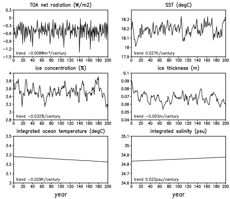
Figure S1. The annual mean of last 200 model years output in the Pliocene simulation
