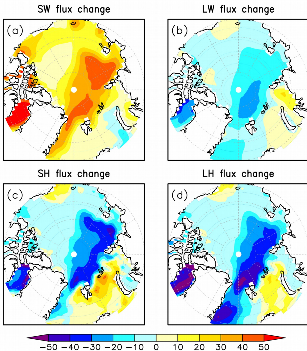
615 Figure 3. Spatial distributions of the Pliocene annual mean heat flux change ( \text{Wm}^{-2} , positive downward) with respect to the preindustrial period over the Arctic Ocean. (a) net shortwave flux, (b) net longwave radiation flux, (c) sensible heat flux, and (d) latent heat flux.
