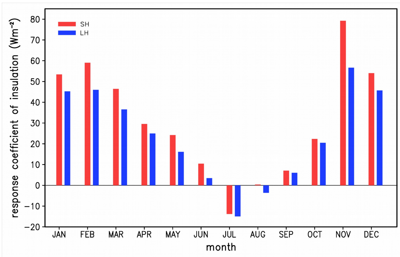
685 Figure 10. The monthly response coefficients (Wm -2 ) of sensible and latent heat fluxes to the insulation effect of sea ice.
