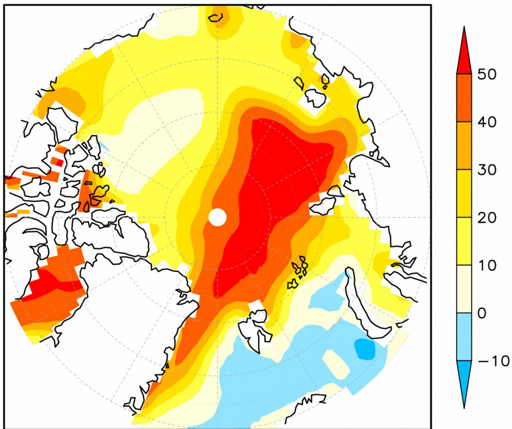
620 Figure 4. Spatial distributions of the Pliocene annual mean net shortwave flux change ( \text{Wm}^{-2} , positive downward) at the surface over the Arctic Ocean caused by albedo effect of sea ice change with respect to the preindustrial period.
