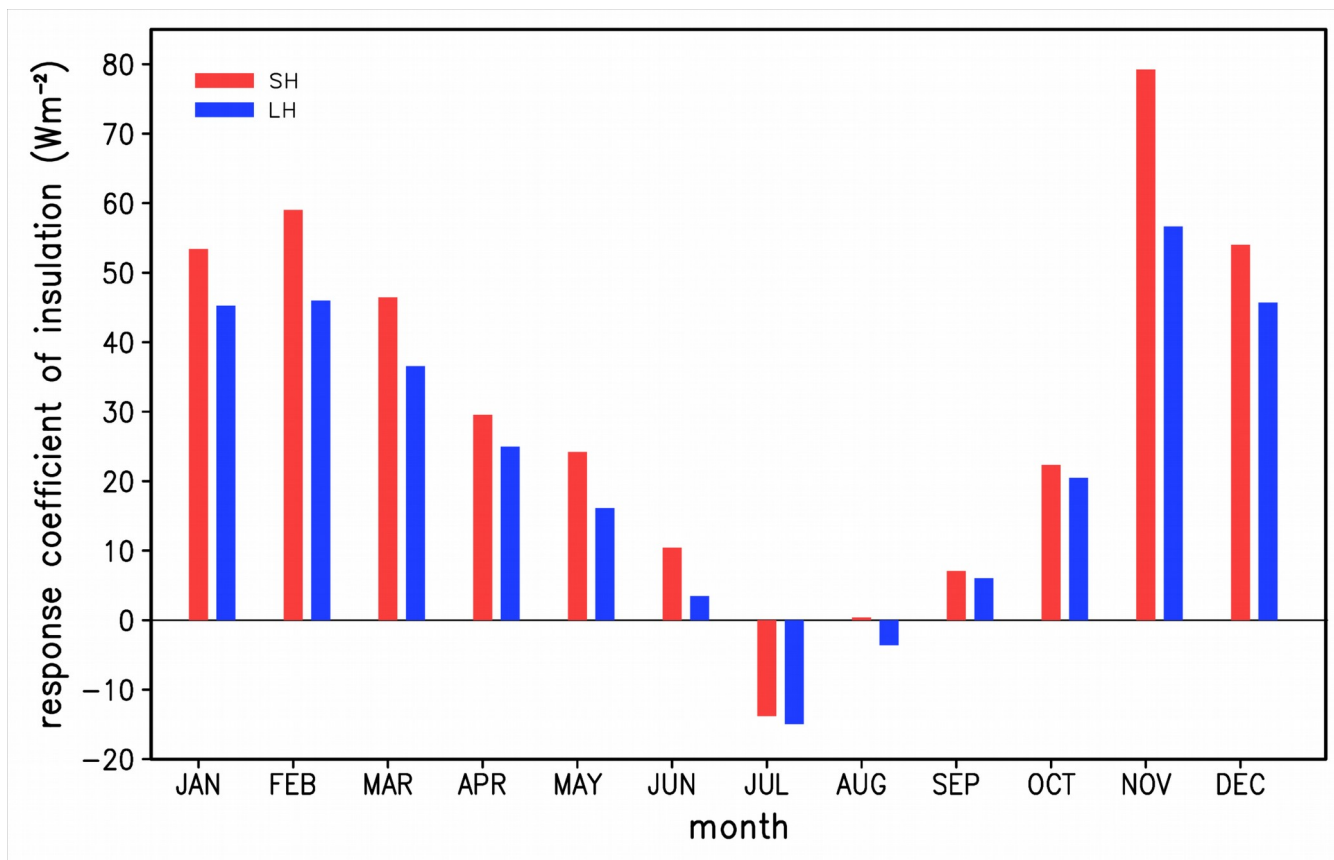
685 Figure 10. The monthly response coefficients ( \text{Wm}^{-2} ) of sensible and latent heat fluxes to the insulation effect of sea ice.
