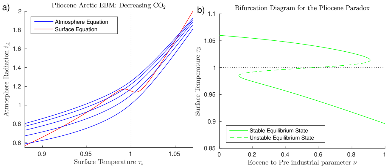
Figure 4. Pliocene Arctic EBM (9)–(10). Parameter values \delta = 0.67 , F_A = 45 Wm -2 , Q = 173.2 Wm -2 , \alpha_W = 0.08 , Z = 9 km. a) CO 2 takes values \mu = 200, 500, 800, 1100, 1400 ppm, from bottom to top on the blue curves, with fixed F_O = 50 Wm -2 on the red curve. The warm equilibrium state \tau_S > 1 disappears as \mu decreases on successively lower blue curves. b) Bifurcation Diagram for the Pliocene Paradox. Here, CO 2 concentration \mu and ocean heat transport F_O decrease simultaneously, with increasing \nu , ( 0 \leq \nu \leq 1 ), as given by Equations (37). As \nu increases, the warm equilibrium solution ( \tau_S > 1 ) disappears in a saddlenode bifurcation, at approximately \nu = 0.91 , corresponding to forcing parameters \mu = 336 ppm and F_O = 50.9 . The equilibrium temperatures at this value of \nu are 3.9C and -26C, and geological time about 4.5 Ma. To the right of this point, only the frozen equilibrium state exists. Between about \nu = 0.12 and \nu = 0.91 , the frozen and warm equilibrium states coexist, separated by the unstable intermediate state.
