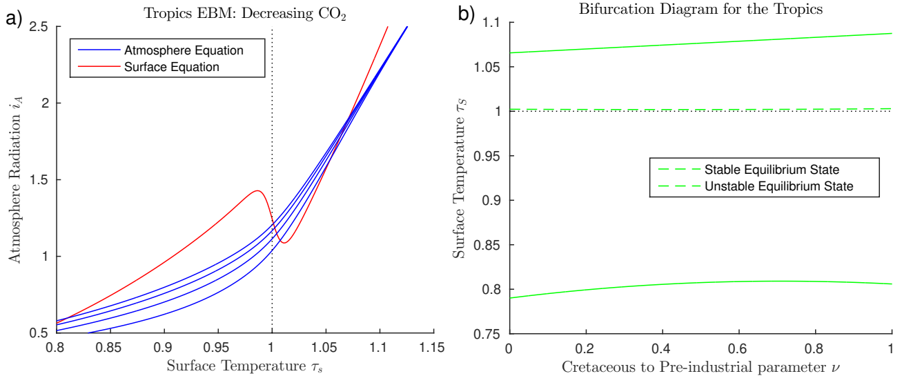
Figure 7. Tropics EBM, using Equations (9)–(10) and parameter values as in Table 2. a) The blue curves represent the atmosphere equilibrium equation for \mu = 300, 600, 900, 1200 , from bottom to top. b) Bifurcation Diagram for the Tropics EBM. Here, \text{CO}_2 concentration \mu and ocean heat transport F_O are both decreasing, with increasing \nu , ( 0 \leq \nu \leq 1 ), as given by Equations (40). As \nu varies, both the warm equilibrium state ( \tau_S > 1 ) and the frozen equilibrium state ( \tau_S < 1 ) persist; there are no saddle-node bifurcations.
