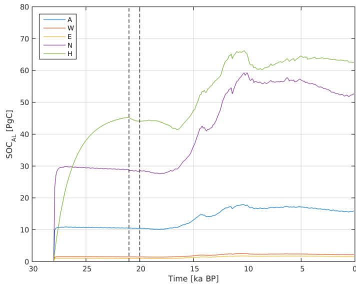
Figure A 13: Simulation set-up for deglacial model runs. Shown is the spinup and fully transient phase of active layer SOC pools for all SOM liability classes (A, W, E, N, H) from the experiment initialization at 28 ka BP to 0 BP. The vertical dashed line at 21 ka BP illustrates the end of the SOC spinup phase, the vertical dashed line at 20 ka BP illustrates the end of the stationary LGM climate forcing. Individual SOC contributions were summed over all permafrost grid cells.
