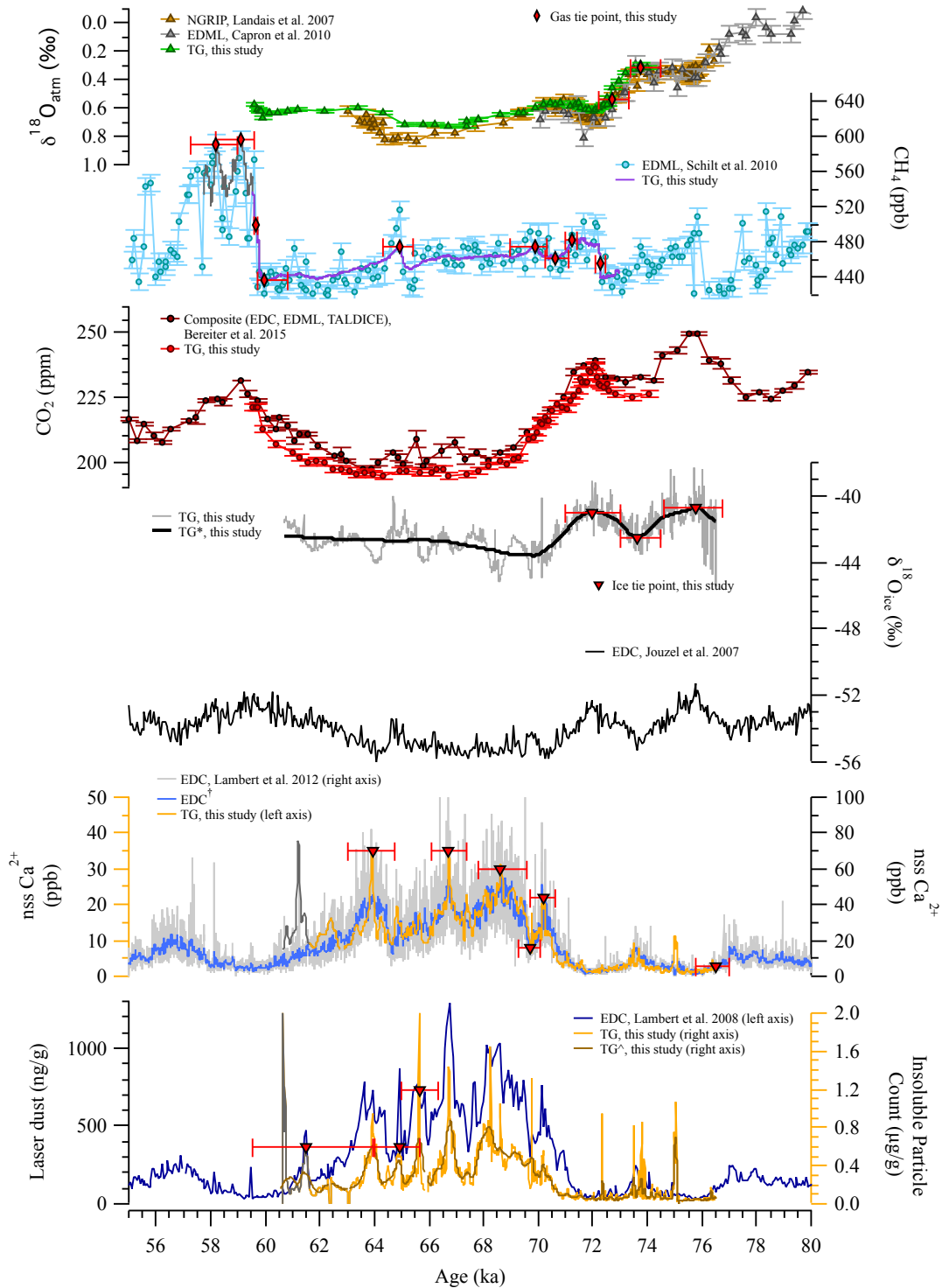
Figure 2 – Measurements of trace gases ( \text{CH}_4 and \text{CO}_2 ), stable isotopes (ice and \text{O}_2 ), insoluble particles, and \text{nss-Ca}^{2+} from the Taylor Glacier ice core on new gas and ice age scales. All ice core data are synchronized to AICC 2012. \text{CH}_4 data from < 4 m depth and dust data from < 40 cm depth are colored dark gray to denote potential contamination by surface cracks. NGRIP = North Greenland Ice Coring Project, TG = Taylor Glacier MIS 5/4 BID cores, EDML = EPICA Dronning Maud Land, EDC = EPICA Dome C, TALDICE = Talos Dome. *, †, and ^ denote smoothing with 5000 point, 100 point, and 50 point LOESS algorithms, respectively.
