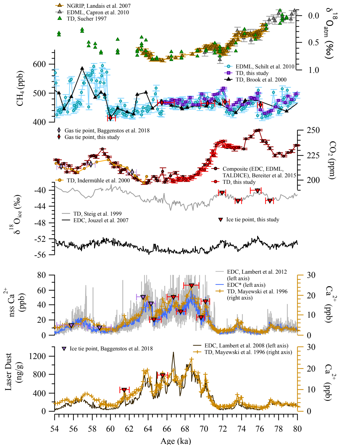
Figure 4 - Measurements of trace gases (CH 4 and CO 2 ), stable isotopes (ice and O 2 ), and Ca 2+ from the Taylor Dome ice core on new gas age and ice age scales. All ice core data are synchronized to AICC 2012. NGRIP = North Greenland Ice Coring Project, TD = Taylor Dome, EDML = EPICA Dronning Maud Land, EDC = EPICA Dome C, TALDICE = Talos Dome. * denotes smoothing with 100 point LOESS algorithm.
