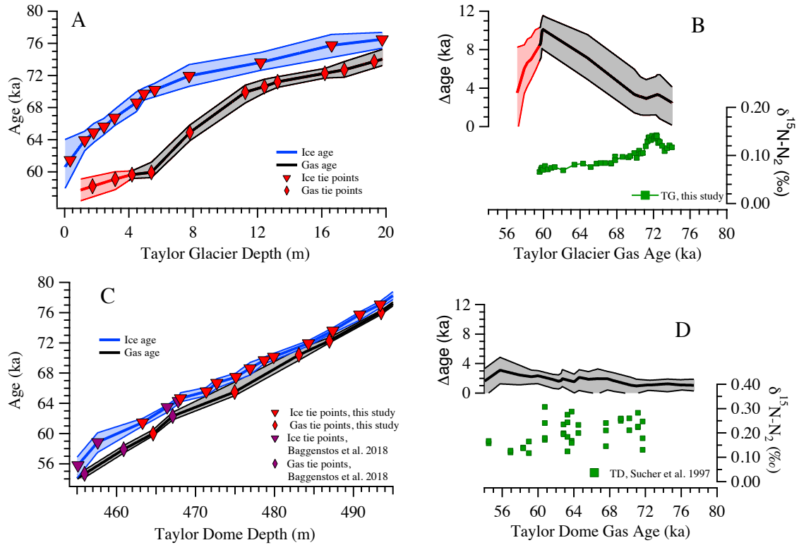
Figure 5 – (A) New Taylor Glacier MIS 5/4 gas and ice age models, and (B) Taylor Glacier \Delta age and \delta^{15}\text{N}-\text{N}_2 . Where age data and \Delta age are plotted in red denote that gas data are from the top 4 m where contamination from surface cracks is possible. (C) Revised Taylor Dome gas and ice age models, and (D) Taylor Dome \Delta age and \delta^{15}\text{N}-\text{N}_2 . \Delta age data are plotted on the gas age scale.
