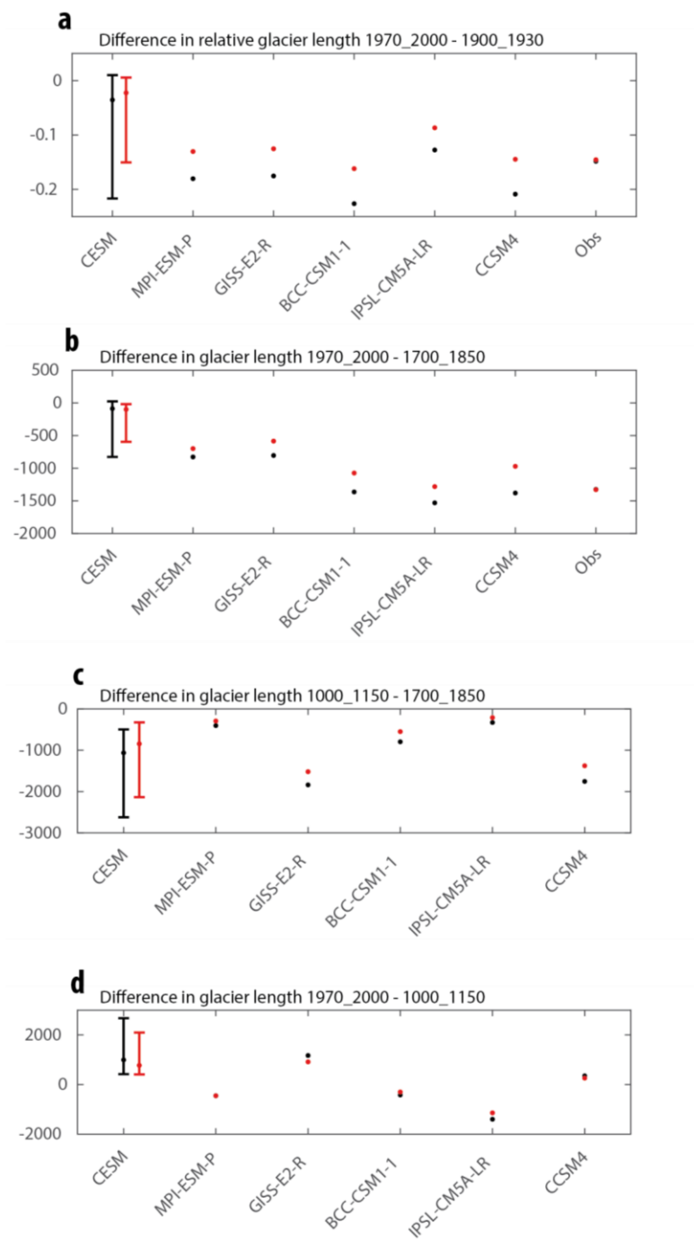
Figure 4. Mean (black) and median (red) of the difference in glacier length between a) 1970-2000 and 1900-1930; b) 1970-2000 and 1700-1850; c) 1000-1150 and 1700-1850; d) 1970-2000 and 1000-1150. No observation is available for panels c and d. For panel b, the average of model results is made only for the glaciers that have observations.
