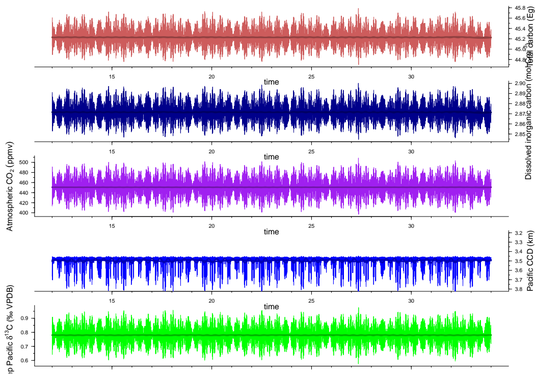
Fig. 2. A time-series with precession as forcing.
