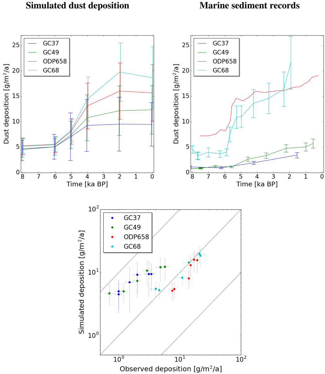
Figure 5. Simulated dust deposition at the position of the marine cores (top left), dust deposition indicated by marine sediment records (Adkins et al., 2006; McGee et al., 2013b) (top right) from 8k to 0k and a comparison of simulated and observed dust deposition (bottom).
