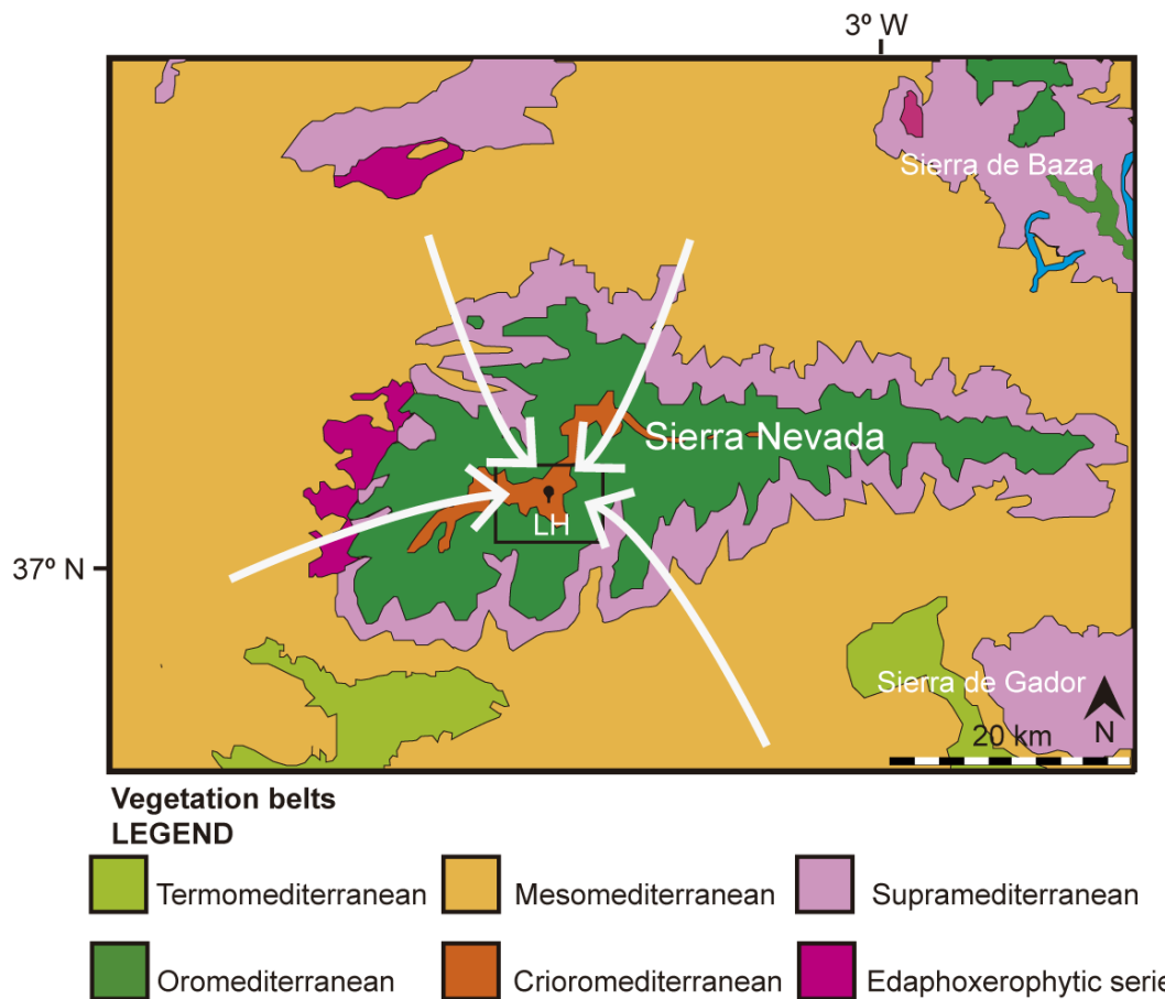
Fig. 1. Modified from Ramos-Román et al., 2018. White arrows indicate possible wind directions.
