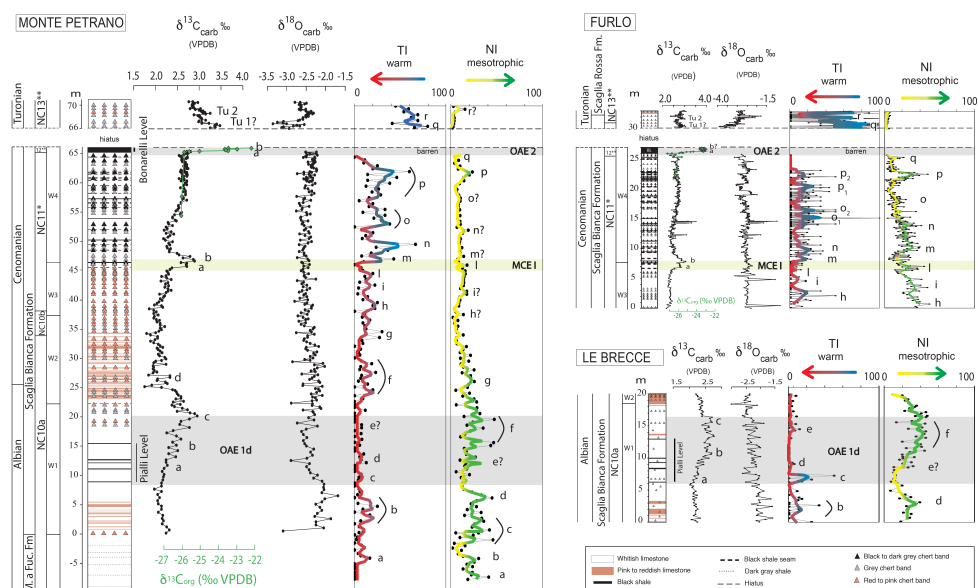
Figure 5: Nannofossil Temperature (TI) and Nutrient (NI) Indices for Monte Petrano, Furlo and Le Breccce sections. TI and NI are reported point by point (in black), and smoothed (TI=blue-red; NI = green-yellow) with a 3pt moving average (Monte Petrano) and 5pt moving average (Furlo and Le Breccce). Lower values of the TI indicate higher temperatures and vice versa. Higher values of the NI indicate higher surface water productivity and vice versa. Litho-, bio-, chemo-stratigraphy is from Gambacorta et al. (2015). Letters “a” to “r” are used to identify peaks and/or interludes of higher TI/NI.
