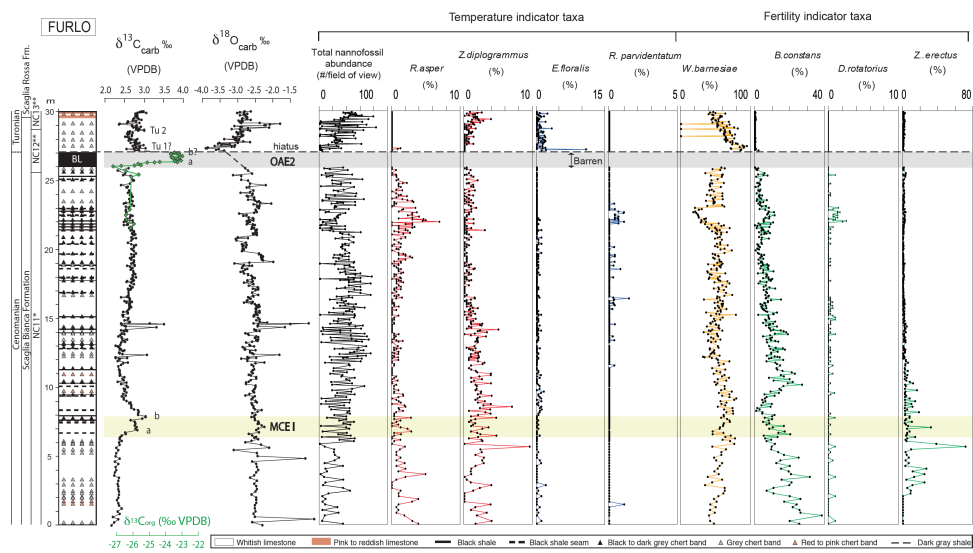
675 Figure 4: Furlo: total calcareous nannofossil abundance, relative (%) abundance of temperature and fertility indicator nannofossil species. The OAE 2 is indicated by a grey band, the MCE I is represented by a yellow band. The stratigraphic framework (litho-, bio-, chemo-stratigraphy) is from Gambacorta et al. (2015).
