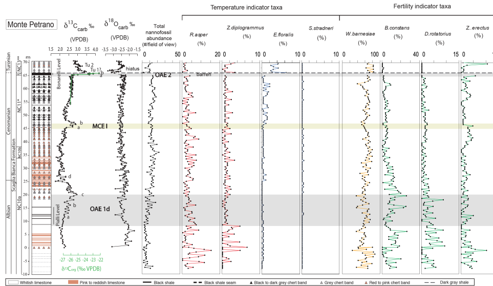
665 Figure 2: Monte Petrano: total calcareous nannofossil abundance, relative (%) abundance of temperature and fertility indicator nannofossil species. The OAE 1d and OAE 2 are indicated by a grey band, the MCE I is represented by a yellow band. The stratigraphic framework (litho-, bio-, chemo-stratigraphy) is from Gambacorta et al. (2015).
