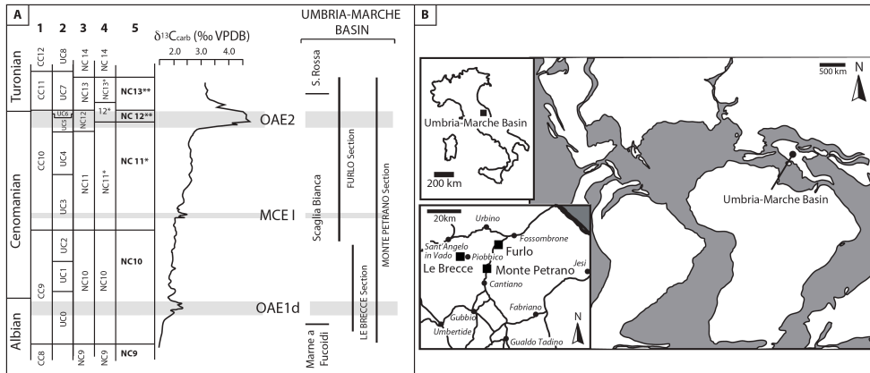
660 Figure 1: A) Stratigraphic ranges of the studied sections plotted against nannofossil biostratigraphy and chemostratigraphy of the late Albian – early Turonian time interval modified after Gambacorta et al. (2015). Nannofossil zones after 1: Sissingh (1977), 2: Burnett (1998), 3: Roth (1978), 4: Bralower et al. (1995), 5: Tsikos et al. (2004), Gambacorta et al. (2015). FO: first occurrence, LO: last occurrence. B) Present-day and paleogeographic location of the studied sections, modified after Gambacorta et al. (2015).
