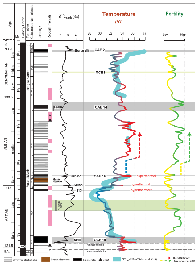
Figure 7: Synthesis of nanofossil-based nutrient and temperature variations reconstructed in the western Tethys. Time scale is after Malinverno et al. (2010, 2012) for the late Barremian – Aptian and after the Geological Time Scale 2012 (Gradstein et al., 2012) for the Albian – Cenomanian. Simplified TEX_{86}^H -SSTs for ocean T > 15^{\circ}C (O’Brien et al., 2018) are reported in light blue. Nanofossil TI and NI trends from the Gault Clay Formation (Kanungo et al. 2018) are represented with coloured dotted lines.
