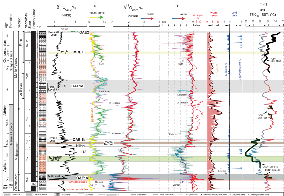
Figure 6: Composite section through the latest Barremian – Cenomanian which includes from bottom to top: i) Cision Core, ii) Piobbico Core, iii) Monte Petrano, Le Brece and Furlo sections. Nannofossil Zones are from Erba (1988), Tiraboschi et al. (2009), Erba et al. (1999), Gambacorta et al., (2015). Smoothed (5pt moving average) \delta^{13}\text{C} and \delta^{18}\text{O} curves and point by point \delta^{18}\text{O} curve include data from the: i) Cision Core (Bottini et al., 2015), ii) Piobbico Core (Tiraboschi et al., 2009 and Bottini et al., 2015), and iii) Monte Petrano (Giorgioni et al., 2012; Gambacorta et al., 2015). Nannofossil Temperature Index (TI) and Nutrient Index (NI) composite curve are calculated following Bottini et al. (2015) and include nannofossil data from: i) the Cision Core (Bottini et al., 2015); ii) the Piobbico Core (Tiraboschi et al., 2009; Bottini et al., 2015); iii) the Monte Petrano, Le Brece and Furlo sections (this work). TI and NI are reported point by point and smoothed (3pt moving average - Monte Petrano, and 5pt moving average - Furlo and Le Brece). Dotted red line is based on R. asper relative abundance. Relative (%) abundance of R. asper and cold-water species ( E. floralis and R. parvidentatum ) are reported. The NI of Furlo and Monte Petrano are both presented in the composite curve (Fig. 6) since are interpreted to reflect local differences. The modified TI (m-TI) takes into account R. asper abundance (%) and it is calibrated with \text{TEX}_{86} -SSTs ( ^{\circ}\text{C} ) recalculated following Kim et al. (2010). \text{TEX}_{86} -SSTs (black lines) include data from: i) DSDP Site 463 (Schouten et al., 2003); ii) DSDP Site 545 (McAnena et al., 2013); iii) ODP Sites 1258 and 1259 (Forster et al., 2007).
