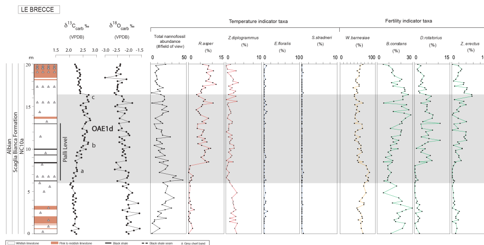
670 Figure 3: Le Brece: total calcareous nannofossil abundance, relative (%) abundance of temperature and fertility indicator nannofossil species. The OAE 1d is indicated by a grey band. The stratigraphic framework (litho-, bio-, chemo-stratigraphy) is from Gambacorta et al. (2015).
