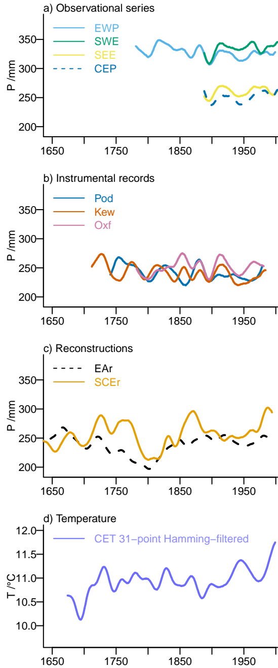
Figure 1. Visualisation of the observation based records for the extended spring season March to July (MAMJJ). We show 31-point Hamming-filtered time series for a) the Met Office Hadley Centre observational precipitation series for England-Wales (EWP), South-West (SWE), South-East (SEE), and Central England (CEP), b) the instrumental precipitation series for Pode Hole (Pod), Kew Gardens (Kew), and Oxford (Oxf), c) the precipitation reconstructions for East Anglia (EAr) and Southern-Central England (SCER), and d) the Central England Temperature (CET) data.
