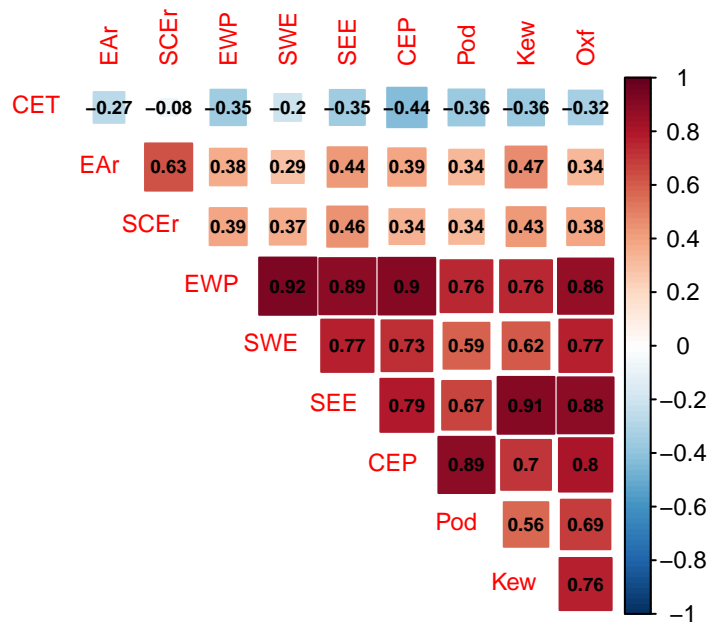
Figure 2. Correlation matrix for complete correlations between the observation or paleo-observation based data sets Central England Temperature (CET), East Anglia precipitation reconstruction (EA r ), Southern-Central England precipitation reconstruction (SCE r ), England-Wales precipitation (EWP), South-West England precipitation (SWE), South-East England precipitation (SEE), Central England precipitation (CEP), PODE Hole precipitation (Pod), Kew Gardens precipitation (Kew), and Oxford precipitation (Oxf). Complete correlations mean that we only use the years 1873 to 1994 for which all records have data. The season for all records is MAMJJ.
