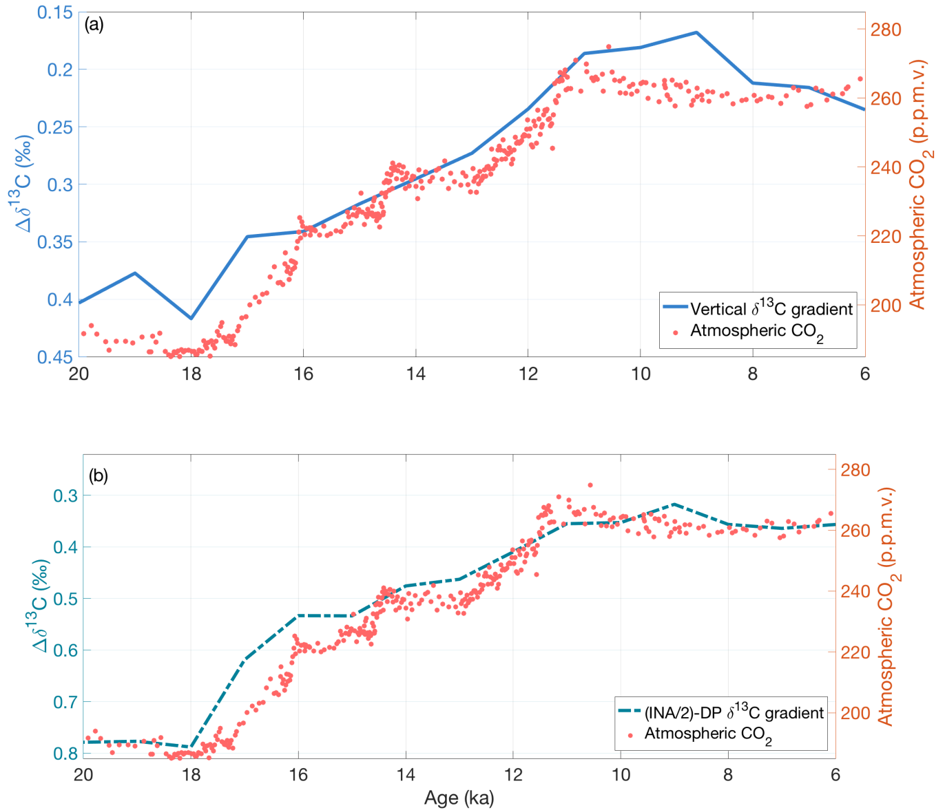
Figure 7. Comparison of atmospheric \text{CO}_2 with (a) the vertical \delta^{13}\text{C} gradient (excluding the data-sparse Indian regions) and (b) \Delta\delta^{13}\text{C}_{(\text{INA}/2)-\text{DP}} . Both gradients have a statistically significant correlation with atmospheric \text{CO}_2 records (red circles, Köhler et al. (2017)). The y-axes for (a) and (b) are scaled differently because \Delta\delta^{13}\text{C}_{(\text{INA}/2)-\text{DP}} scales the intermediate North Atlantic stack by half before subtracting the deep Pacific stack while the \delta^{13}\text{C} gradient is the difference between the Atlantic-Pacific intermediate and deep stacks.
