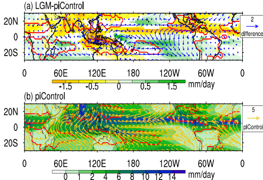
Figure 3 (a) JJA mean precipitation (shading) difference and surface wind (vectors) difference between LGME and piControl, and (b) the climatology of JJA mean precipitation (shading) and surface wind (vectors) derived from piControl. The red lines enclose the monsoon domains. The thick black lines in (a) denote the coastal lines in LGME provided by CMIP5/PMIP3, and the
