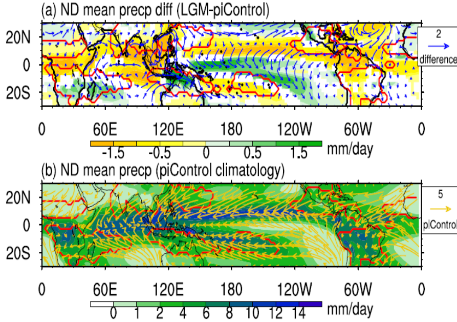
Figure 6 (a) ND mean precipitation (shading) difference and surface wind (vectors) difference between LGM and piControl, and (b) the climatology of ND mean precipitation (shading) and surface wind (vectors) derived from piControl. The red lines enclose the monsoon domains. The thick black lines in (a) denote the coastal lines in LGM provided by CMIP5/PMIP3, and the thin black lines denote the coastal lines in piControl. Only those areas where signal-to-noise ratio exceeds one are plotted in (a).
