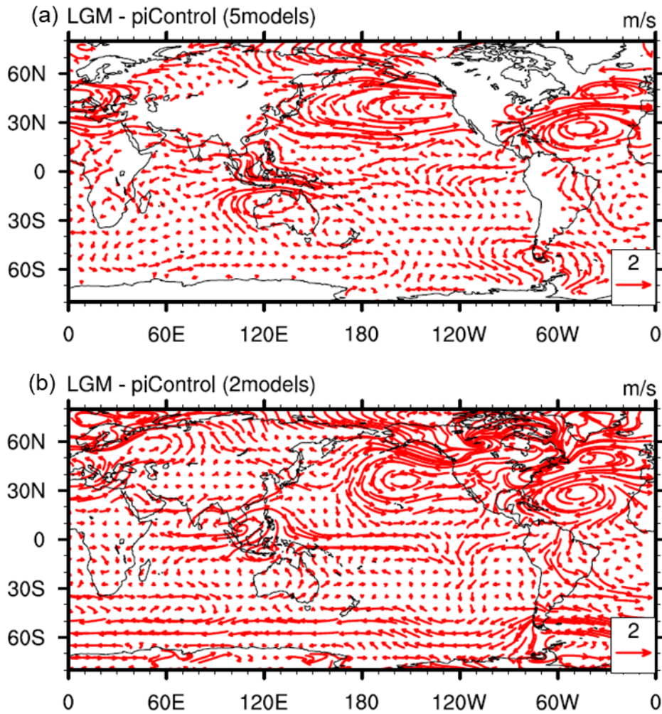
747 Figure 14 DJF mean 850hPa wind differences between LGME and piControl derived from (a) 748 the five models and (b) the two models. Only those areas where signal-to-noise ratio exceeds one 749 are plotted.
