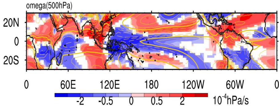
Figure 7 The difference of the ND mean vertical velocity at 500 hPa between LGM and piControl (in shading) and the corresponding climatology derived from piControl (yellow contours). The thick black lines denote the coastal lines in LGM provided by CMIP5/PMIP3, and the thin black lines denote the coastal lines in piControl. Only those areas where signal-to-noise ratio exceeds one are plotted in the difference pattern.
