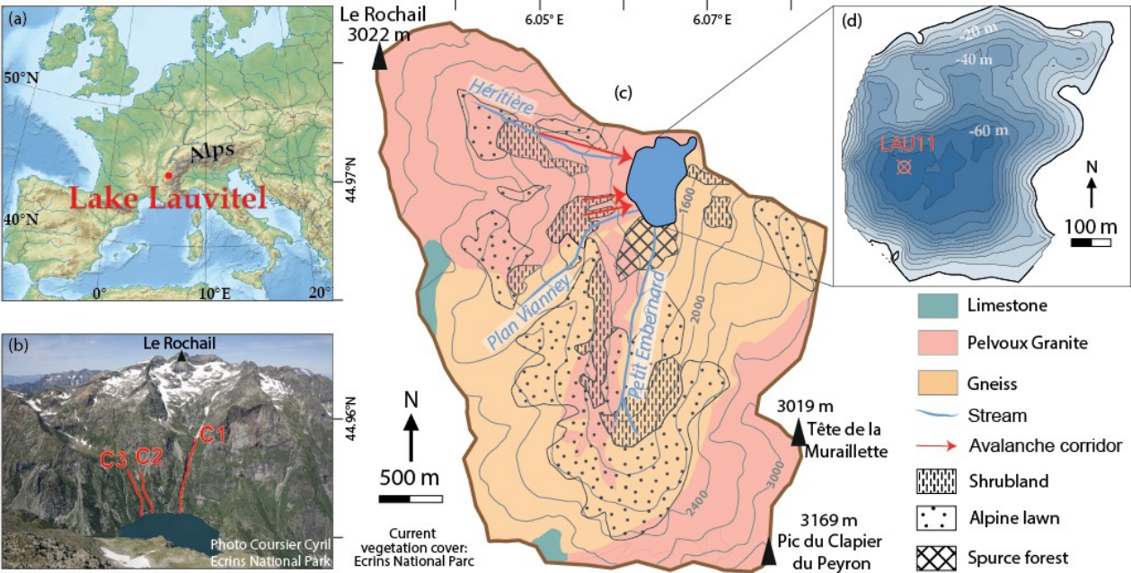
Figure 1: a) Location of Lake Lauvitel in the western Alps. b) Photograph towards the west of the lake watershed exhibiting three avalanche corridors. c) Simplified geological maps of Lake Lauvitel watershed and current vegetation cover. d) Lake bathymetry and position of LAU11 sediment core.
