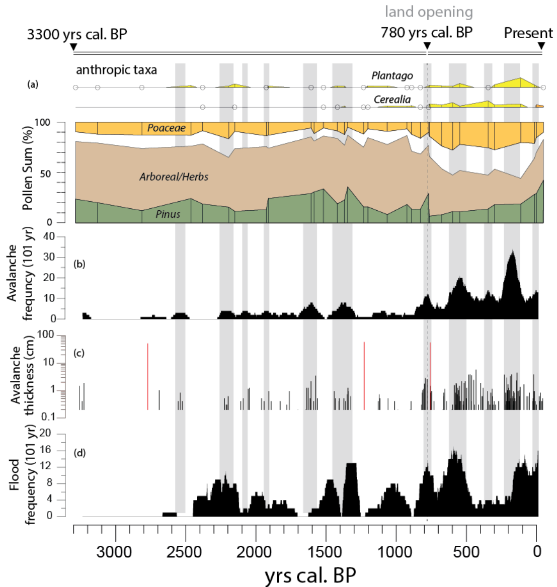
Figure 7: Lake Lauvitel extreme event erosion pattern versus pollen data. (a) Anthropogenic taxa found in pollen analysis, and pollen sum (%) of Poaceae , Pinus , and ratio between Arboreal/Herbs pollen. (b) Lauvitel avalanche chronicle averaged on 101 year. (c) Lake Lauvitel avalanche thickness in centimeters (red bars correspond to the three thickest avalanche deposits). (d) Lake Lauvitel flood chronicle (averaged on a 101 year). Grey band indicate periods of higher avalanche activity.
