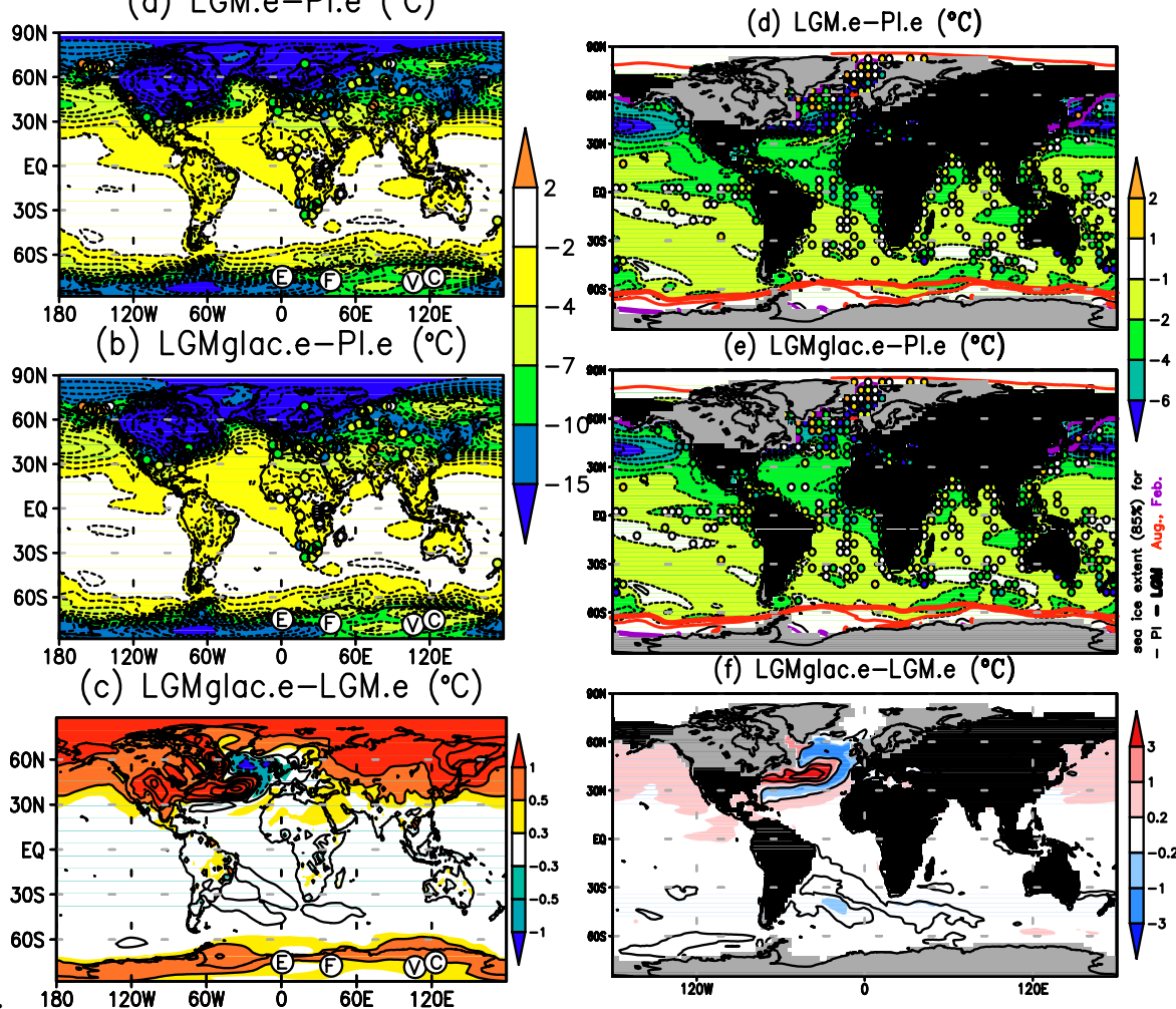
5 Figure 12: Difference of surface temperature at 2 m height: (a) LGM.e–PI.e, (b) LGMglac.e–PI.e, and (c) LGMglac.e–LGM.e. Coloured circles represent reconstructed temperature change by pollen proxy archives (Bartlein et al., 2011). Circled letters in Antarctica represent four ice core locations: E for EDML, F for Dome Fuji, V for Vostok, and C for Dome C. Sea surface temperature (SST) changes: (d) LGM.e–PI.e, (e) LGMglac.e–PI.e, and (f) LGMglac.e–LGM.e. Purple and red lines in (d) and (e) are 85 % sea ice concentration in February and August for PI (thin) and LGM (thick), respectively. Coloured circles represent MARGO SST
