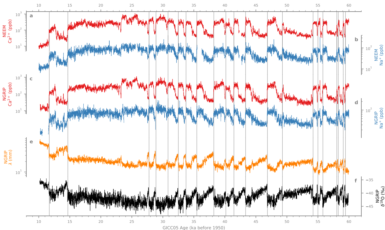
Figure 1. Investigated records from the NEEM (a, b) and NGRIP ice cores (c-f). (a, d) show the new aerosol records of \text{Ca}^{2+} (a, c) and \text{Na}^{+} (b, d) alongside the NGRIP layer thickness, \lambda (e) and ice \delta^{18}\text{O} records (f). All records are shown as decadal averages on their respective version of the GICC05 age scale relative to 1950 (Svensson et al., 2008; Rasmussen et al., 2013). The vertical lines mark the investigated interstadial onsets as given by Rasmussen et al. (2014). Note that the vertical scales for the aerosols and annual layer thickness are logarithmic.
