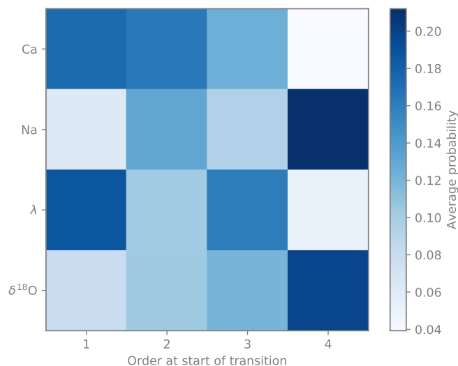
Figure 5. Combined order statistics for the onset of the transition. The colors indicate the probability of observing the onset of the transition in the parameter on the y-axis at the position on the x-axis. This illustrates that during the onset of the DO-warming, the changes in accumulation and \text{Ca}^{2+} concentrations about equally likely occur first whereas the transitions in \text{Na}^+ and \delta^{18}\text{O} about equally likely occur last.
