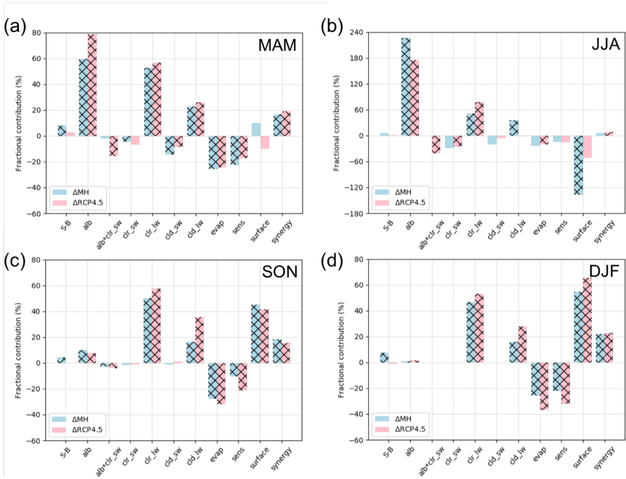
Figure 10 Fractional contribution of individual processes to the model spread in the simulated surface temperature change (%) over the ocean (north of 60°N) for \Delta\text{MH} and \Delta\text{RCP4.5} : (a) spring (March-April-May); (b) summer (June-July-August); 5 (c) autumn (September-October-November); and (d) winter (December-January-February) means. The sum of the bar graphs in the same color for each plot adds up to 100%. The hatching indicates the contribution is statistically significant at the 10% level. All 10 models listed in Table 2 are used. See Table 3 for the interpretation of each component. Note that the vertical scale for (b) is three-fold larger than in the other plots.
