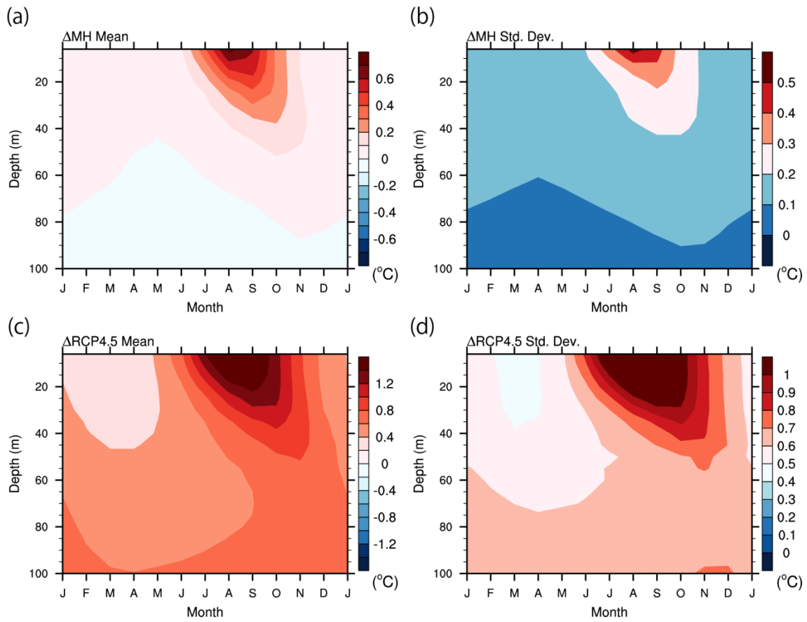
Figure 8 Same as in Fig. 6 but for the upper ocean temperature change (°C) (north of 60°N). 9 models except for FGOALS-g2 listed in Table 2 are used.
