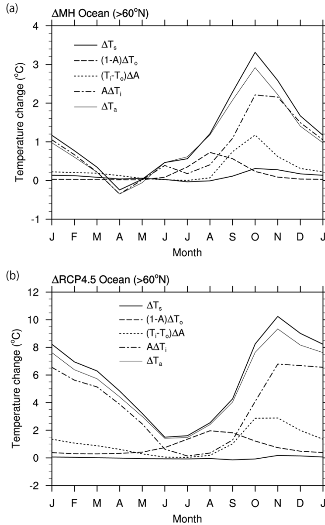
Figure 7 Contribution of the individual components to the surface temperature change (°C) over the ocean (north of 60°N): (a) ΔMH; and (b) ΔRCP4.5. The surface temperature change is decomposed into the components of the SST change ( (1 - A)\Delta T_o ), sea ice concentration change ( (T_i - T_o)\Delta A ), and sea ice surface temperature change ( A\Delta T_i ). Simulated surface temperature ( \Delta T_s ) and surface air temperature changes ( \Delta T_a ) are also plotted for reference. Only 5 models (bcc-csm-1, CCSM4, CNRM-CM5, IPSL-CM5A-LR, and MRI-CGCM3) are used.
