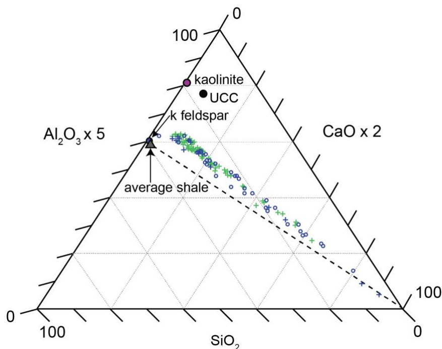
5 Figure 4: Ternary diagram (Brumsack, 1989) displaying the relative contributions of clay ( \text{Al}_2\text{O}_3 ), quartz ( \text{SiO}_2 ), and carbonate ( \text{CaO} ) within all samples. Lower variability mudstone interval (LVMI) samples are indicated by green crosses and higher variability mudstone interval (HVMI) samples are marked by blue symbols, TOC-rich samples ( \text{TOC} > 10 \text{ wt } \% ) are indicated by blue circles and TOC-lean samples ( \text{TOC} < 10 \text{ wt } \% ) are indicated by blue crosses. Axes are scaled to improve display of the data. Average shale (Wedepohl, 1991), upper continental crust (UCC; Rudnick and Gao, 2003), k-feldspar and kaolinite are plotted for reference. Dashed line shows the average shale-carbonate mixing line.
