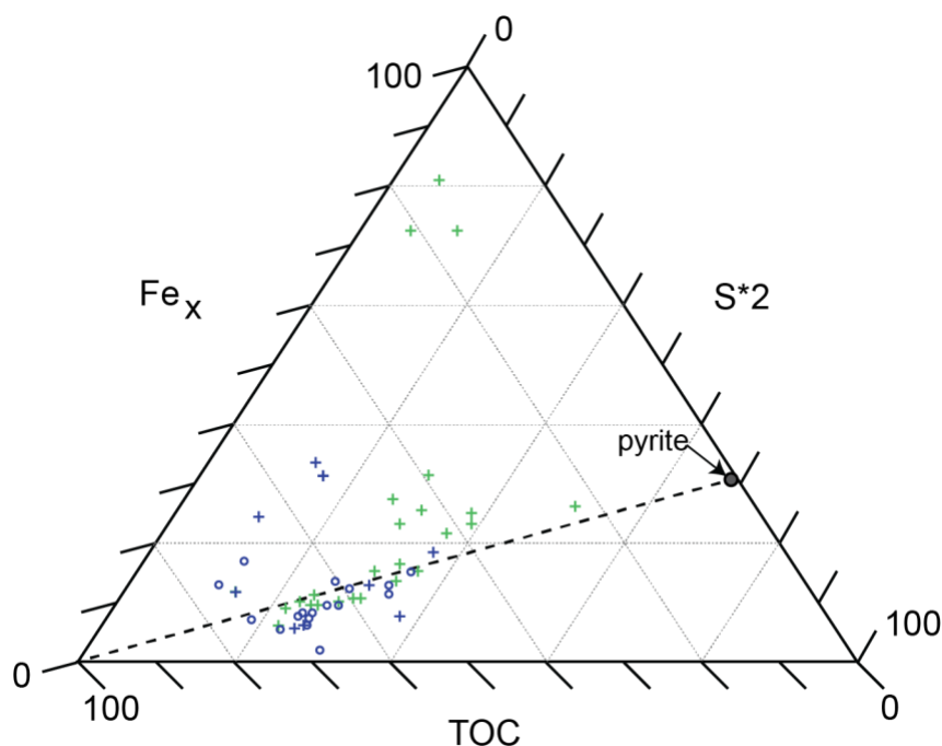
5 Figure 7: Fe_x -TOC-S Ternary diagram (after Dellwig et al., (1999); Hetzel et al., (2011)). See text for comments on Fe_x calculation. Dashed line represents TOC-pyrite mixing line. Lower variability mudstone interval (LVMI) samples are indicated by green crosses (three samples nearest to the Fe_x corner represent the diagenetically overprinted samples that were excluded from the interpretation). Higher variability mudstone interval (HVMI) samples are marked by blue symbols, TOC-rich samples (TOC > 10 wt %) are indicated by blue circles and TOC-lean samples (TOC < 10 wt %) are indicated by blue crosses.
