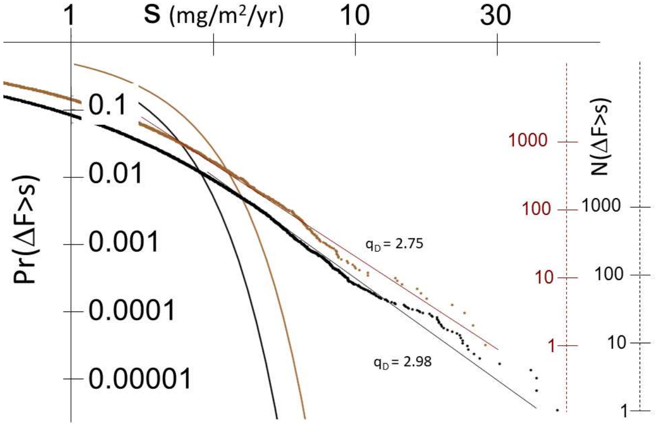
Figure 6a: The probability distribution \text{Pr}(\Delta F > s) of random changes in dust flux ( \Delta F ) exceeding a fixed threshold s ; in time at 25 year resolution (brown, 32,000 points), and in depth at 1cm resolution (black, 251,075 points corresponding to the last 400 kyrs). The frequency scales at the right give the number ( N ) of jumps in each of the series that exceeds the threshold s . The straight lines indicate power law probability tails with exponents q_D indicated. Also shown (parabolas) are the Gaussians with the same mean and standard deviations. In time, the maximum change in flux corresponds to about 28 standard deviations (i.e. to a Gauss probability \approx 10^{-91} ), in depth, to 51 standard deviations (i.e. to p \approx 10^{-455} ). On the right, we provide axes giving the actual number of flux increments that exceed s , brown for the fluctuations in time, black for those in depth.
