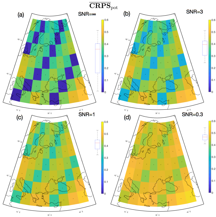
Figure 9. Local \overline{\text{CRPS}}_{\text{pot}} between reconstructed temperature field and target field for the verification period. The boxplots left of the color bars indicate the distribution of grid point correlation coefficients. \beta = 0.75 .
