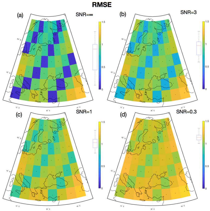
Figure 8. Local root-mean square error (RMSE) between reconstructed temperature field and target field for the verification period. The boxplots left of the color bars indicate the distribution of grid point correlation coefficients. \beta = 0.75 .
