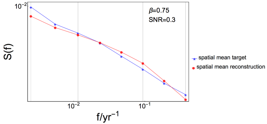
Figure 6. Log-log plot showing log-binned power spectra of spatial mean target (blue) and reconstruction (red) for one experiment. Vertical, gray lines mark the frequency ranges used to estimate bias of variance as referred to in Sect. 4.4.
