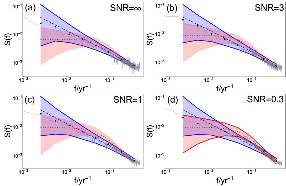
Figure 5. Mean raw and log-binned PSD for the spatial mean reconstruction (gray curve and dots, respectively), generated from \beta_{\text{target}} = 0.75 and different SNR. Colored shadings and dashed/dotted lines indicate 95% confidence range and the ensemble mean, respectively, for a Monte Carlo ensemble of fGn with \beta = 0.75 (blue) and of AR(1) processes with \alpha estimated from BARCAST (red). The confidence ranges found consistent with the data are drawn with solid lines.
