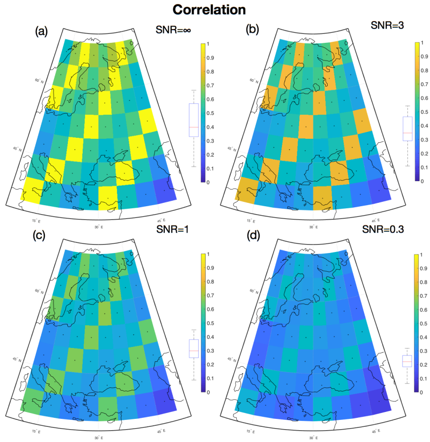
Figure 7. Local correlation coefficient between reconstructed temperature field and target field for the verification period (ensemble mean). The boxplots left of the color bars indicate the distribution of grid point correlation coefficients. \beta = 0.75
