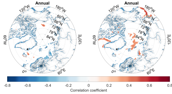
Figure 14. Maps showing the d_{\text{XS}} -SST (left) and d_{\text{XS}} -SIC correlation coefficients between annually averaged data from RECAP and ERA-Interim covering the 1980-2014 period ( p < 0.05 ).
