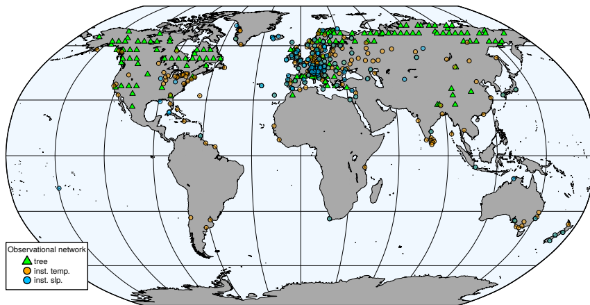
Figure 1. The observational network in 1904, before quality check.
