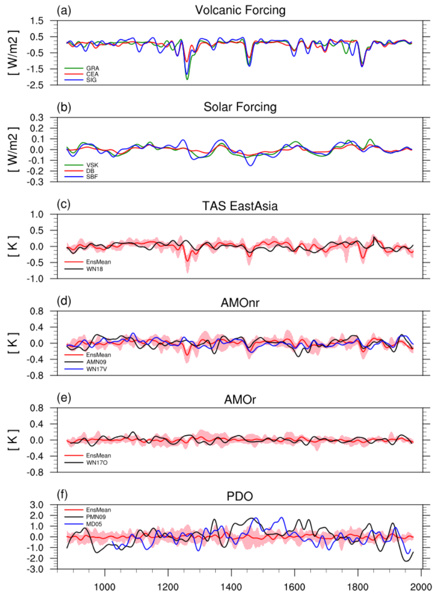
Figure 7: Timeseries of (a) volcanic forcing, (b) solar forcing, (c) surface temperature over East Asia, (d) AMO index without subtracting the global SST (AMO nr ), (e) AMO index after subtracting the global SST (AMO r ), and (f) PDO index, all are annual mean values, passed through a 30-year low pass filter and truncated to remove filter end effects. Model simulations in (c)–(f) are given as the mean (red line) and spread (pink shading) of the 7 GCMs. Model simulations for surface temperature, AMO and PDO are compared with the available reconstructed data (black and blue lines).
