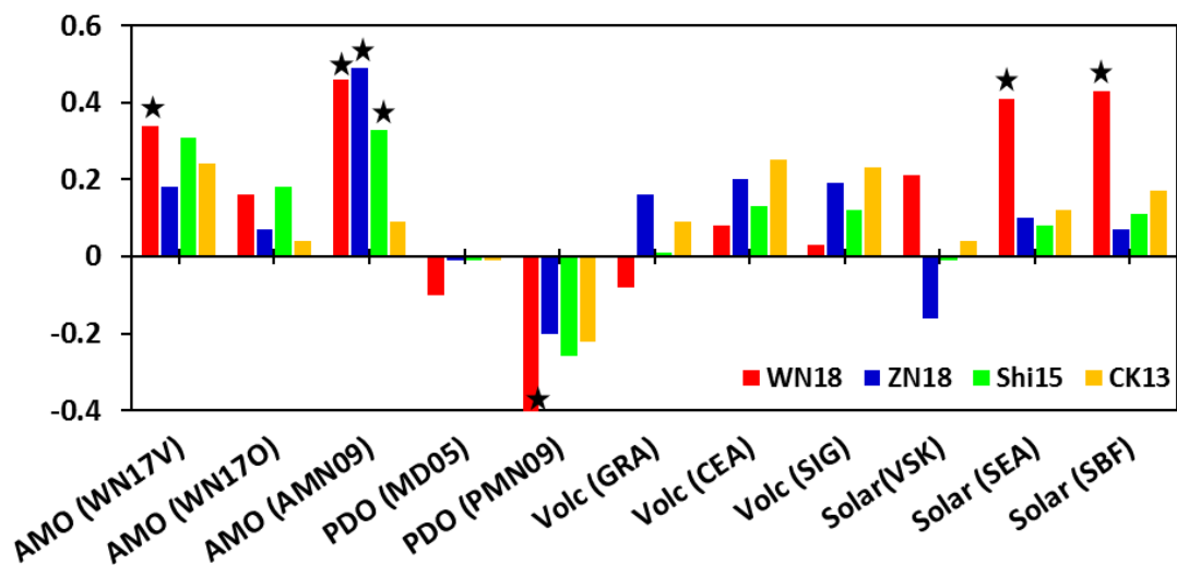
Figure 3: Correlation of TAS reconstructions with AMO, PDO, volcanic forcing and solar forcing reconstructions. The bars marked with 'star' are significance at 95% level using a two-tailed student t-test.
