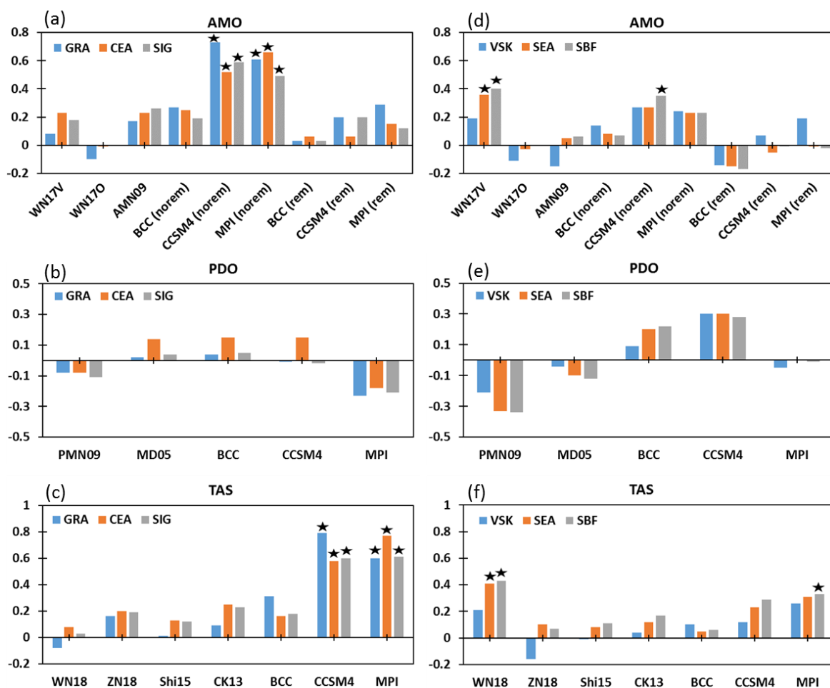
Figure 4: The correlations of (a) AMO, (b) PDO and (c) TAS with volcanic and solar forcing (models and reconstructions) data. (a-c) for volcanic forcing and (d-f) for solar forcing. The bars marked with ‘star’ are significance at 95% level using a two-tailed student t-test.
