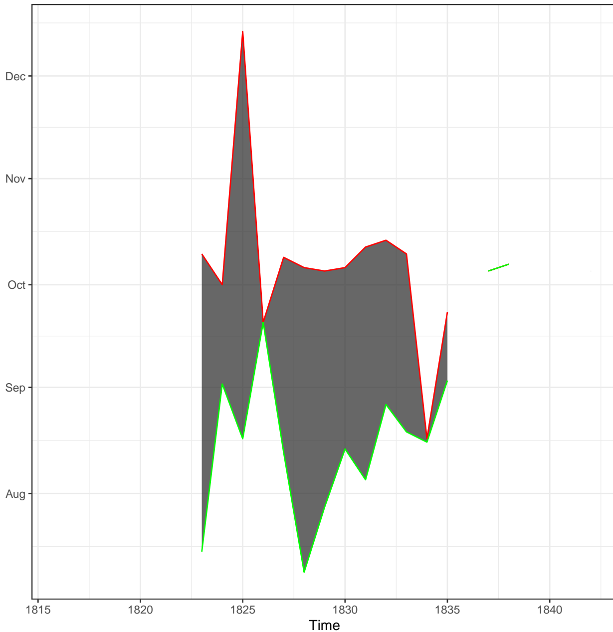
Figure 7. Reports of ague and fever in the Shirley Plantation document during the period 1823–1842. Data for 1839–841 has not been generated yet. There are two decades of data, minus the missing years. Onset of symptoms indicate that the mean daily temperatures had been above 18° Celsius (64.4° Fahrenheit) long enough for the sporogical cycle of Plasmodium to complete in the host Anopheles mosquito.
